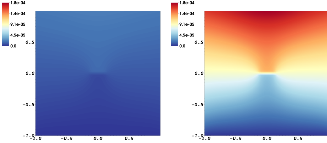
FIGURE 4. Initial y -displacement field and final y -displacement field after four Newton iterations at M = 5 .
