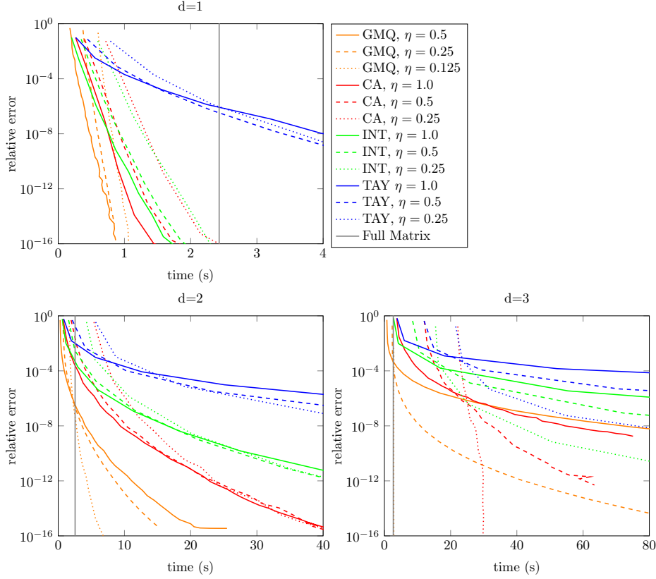
FIG. 5. Time required to compute B_{\mathcal{H}} for N = 10,000 , \phi = \phi_{IMQ,\alpha} , \alpha = N^{-1/d} , for d = 1, 2, 3 .
