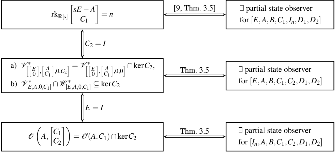
Figure 3: Simplified conditions for the existence of a partial state observer in the cases C_2 = I_n and E = I_n , and comparison with [9].
