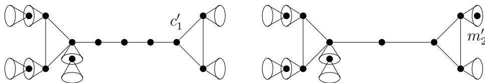
FIGURE 3.2. On the left the graph D_3 of case k = 5 and \ell = 3 where the vertex c'_1 does not have enough neighbours, and on the right the graph D'_3 where the vertex m'_2 does not have enough neighbours.
