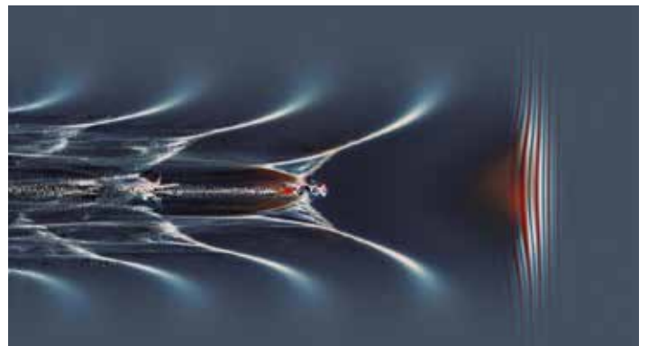
Figure 2 Particle-in-cell simulation of a laser-driven plasma wave. The intense laser travels to the right and induces a charge separation by pushing plasma background electrons to the side. A bubble-like plasma cavity is formed, in which an electron bunch can be trapped and accelerated.
