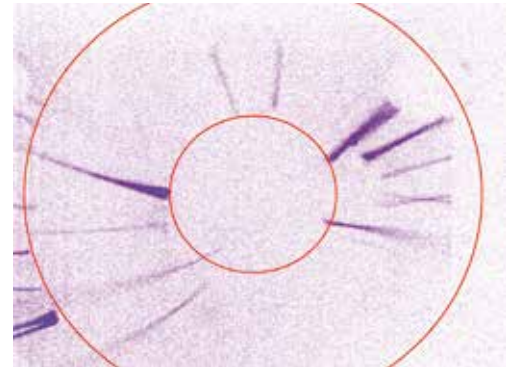
Figure 3 Dark current measured at screen 3GUN (1.5 m downstream of the cathode). The RF gun is operated with 5 MW forward power corresponding to a 53 MV/m field gradient on the cathode and with a solenoid current of 309 A (0.182 T). The total dark current is 6 \mu\text{A} . The circles approximately indicate the rim of the cathode plug (outer circle) and the cathode's \text{Cs}_2\text{Te} thin film (inner circle).
