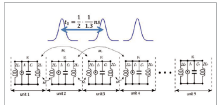
Figure 1 Coupled circuit model with nine units driven by a Gaussian pulse
