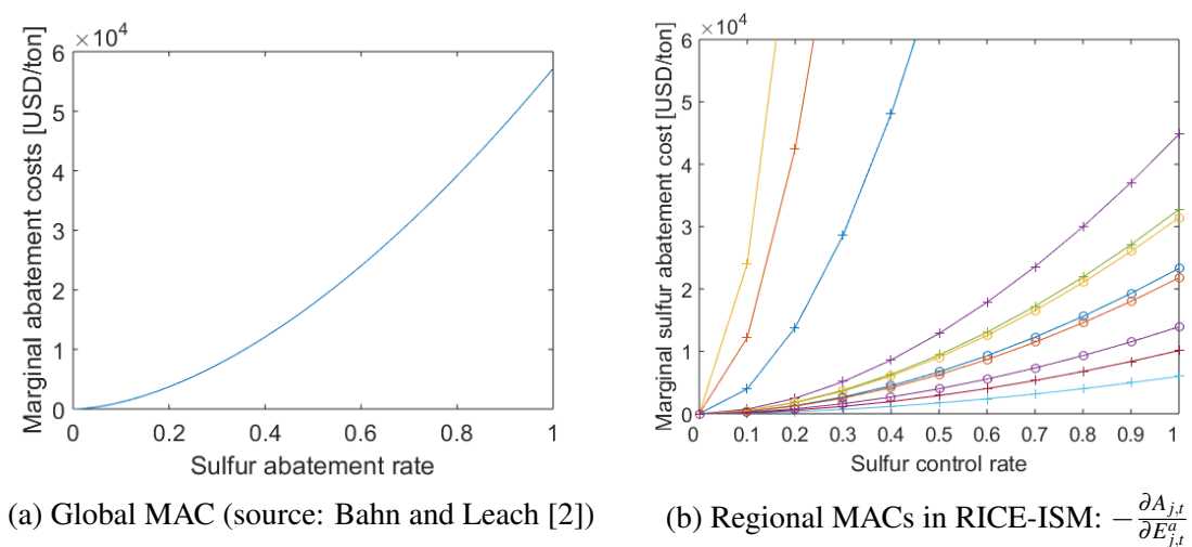
Fig. 3.8 Marginal sulfur abatement costs
