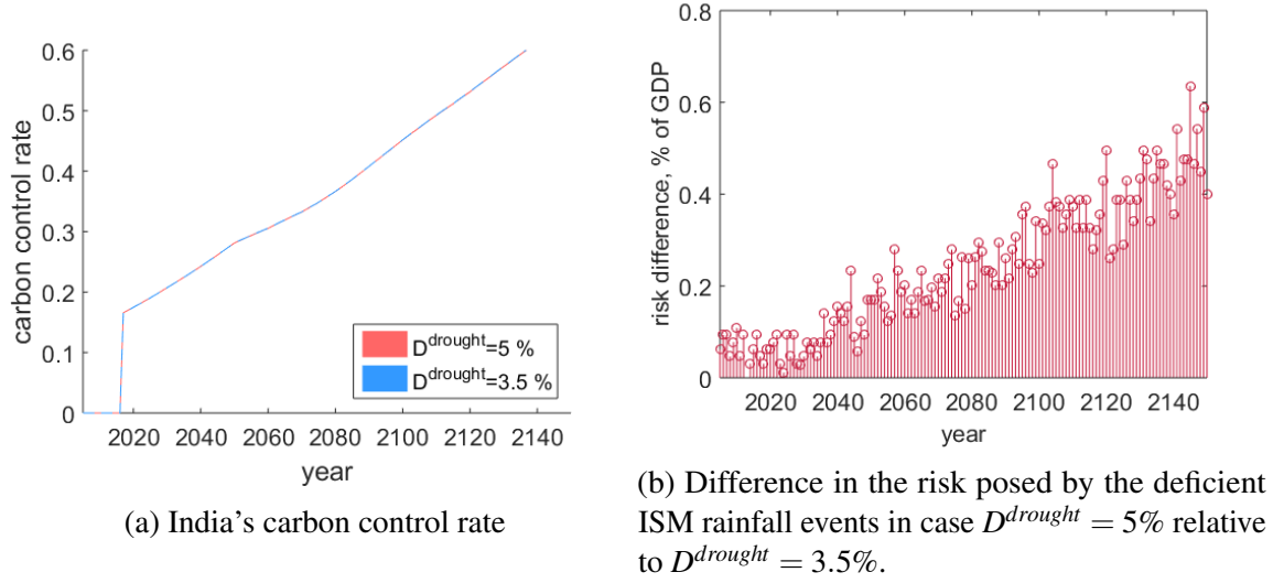
Fig. 2.16 Optimal solution for alternative drought-related damage costs
