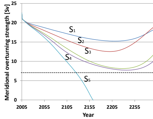
(b) Possible trajectories of the overturning strength
