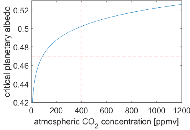
Fig. 2.6 Critical level of planetary albedo in dependence of atmospheric CO 2 concentration (blue curve). If the current values of planetary albedo over India (horizontal red dashed line) and of the atmospheric CO 2 concentration (vertical dashed red lines) alter such that both (i.e. the intersection of the red lines) transgress the critical level, then the ISM switches into a weak hydrological cycle.
