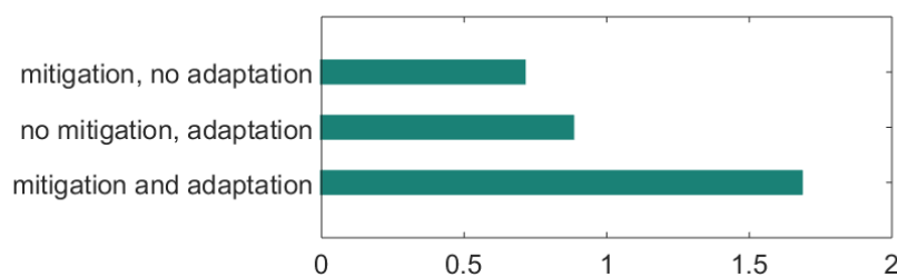
Fig. 3.15 Welfare gains for alternative emissions control and adaptation policies: percentage change relative to the business-as-usual scenario
