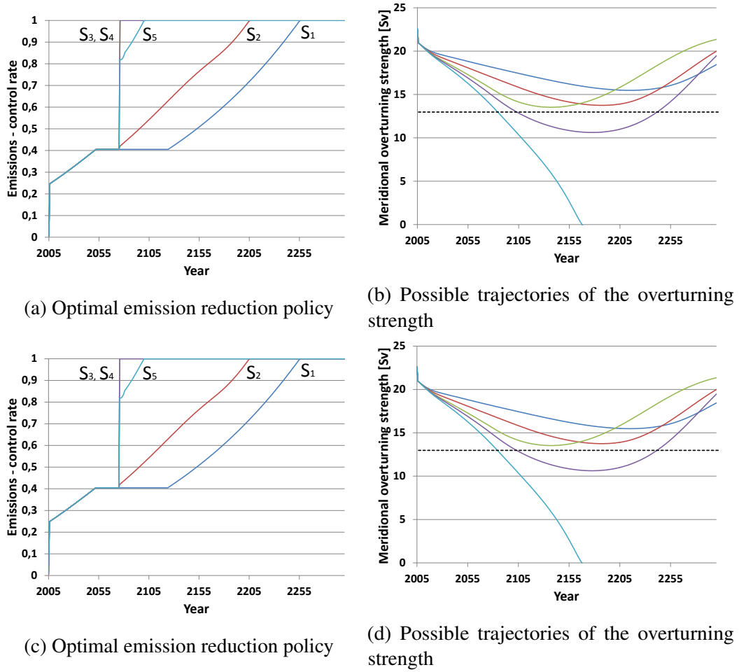
Fig. 1.D.3 Sensitivity of the results with respect to higher value of critical weakening, m_{crit} = 13 Sv
