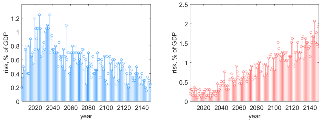
(a) The risk posed by the excess ISM rainfall, where D^{flood} = 5\% (b) The risk posed by the deficient ISM rainfall, where D^{drought} = 5\%
