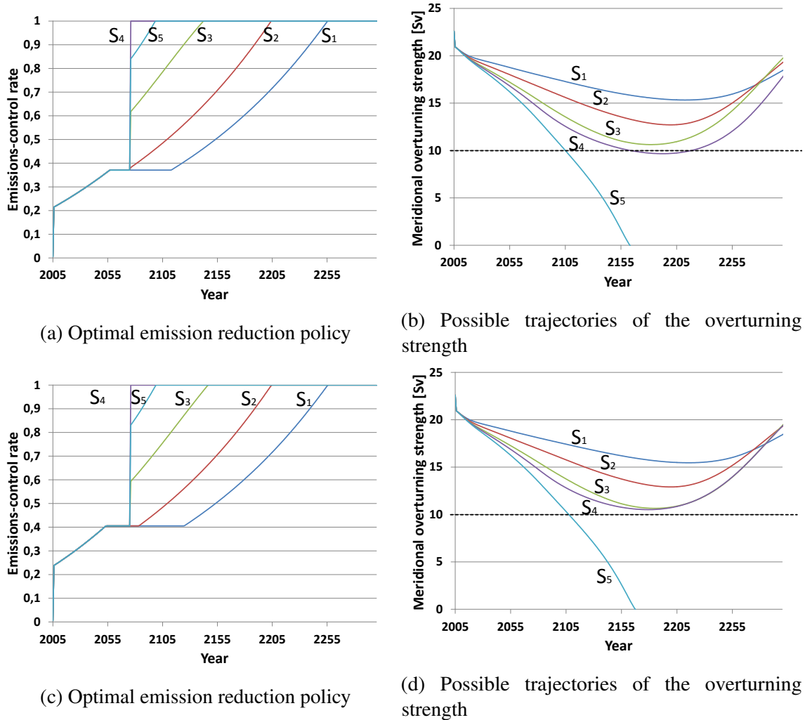
Fig. 1.8 Sensitivity of the results with respect to lower damage costs caused by a critical weakening of a THC, i.e. d_m = 0.015
