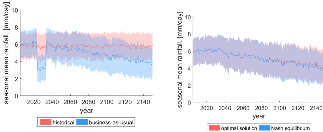
(a) Business-as-usual solution versus historical data (b) Optimal solution versus Nash equilibrium
