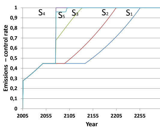
(a) Optimal emission reduction policy
