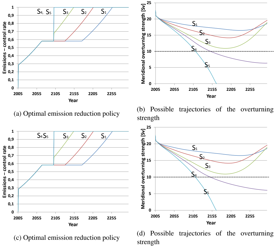
Fig. 1.12 Sensitivity of the results with respect to learning later, i.e. in 2100
