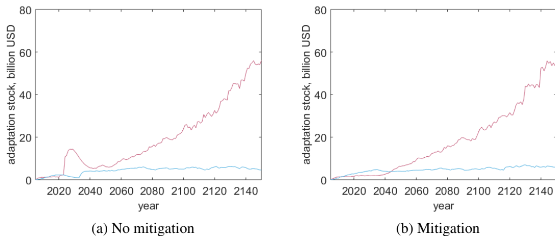
Fig. 3.13 Evolution of adaptive capital stocks K_t^{drought,adapt} (red line) and K_t^{flood,adapt} (blue line) under alternative emissions control policies
