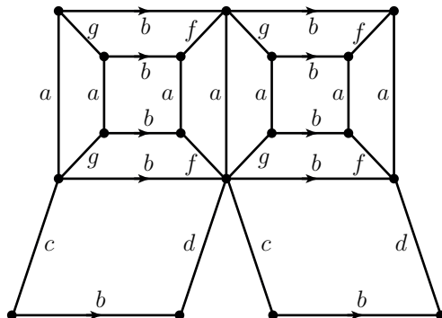
Figure 3: An (infinite) planar Cayley graph, corresponding to the presentation \langle a, b, c, d, f, g \mid a^2, c^2, d^2, f^2, g^2, (af)^2, (ag)^2, abab^{-1}gbfb^{-1}, cdbd^{-1} \rangle , with a separating edge b which is not an involution.
