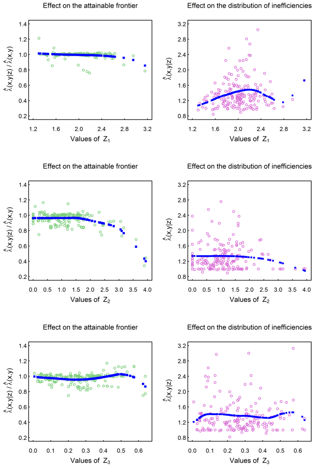
Legend Figure 2: The relationship of quality measures with the production process. Scatterplot of the ratios R = \lambda(x,y|z)/\lambda(x,y) against Z (left panel); scatterplot of the conditional efficiencies \lambda(x,y|z) against Z (right panel). The mean values of the corresponding nonparametric regressions are depicted with dark blue squares. Z_1 = patient satisfaction, Z_2 = risk-adjusted mortality, Z_3 = patient radiation exposure.
