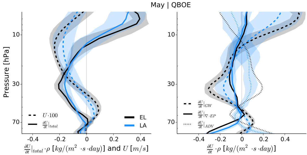
Figure 4.12: Vertical profile of zonal wind U and its tendency \frac{\partial U}{\partial t} for QBOE in May of the second year for El Niño (black) and La Niña (blue) conditions. Lines show the ensemble means and shading indicates the range of two standard deviations ( 2\sigma ). Left panel: Zonal wind (dashed), scaled by a factor 100, and total tendency \frac{\partial U}{\partial t}|_{total} (solid). Right panel: Tendency components of resolved waves \frac{\partial U}{\partial t}|_{\nabla \cdot EP} (solid), gravity waves \frac{\partial U}{\partial t}|_{GW} (dashed) and advection \frac{\partial U}{\partial t}|_{ADV} (dotted).
