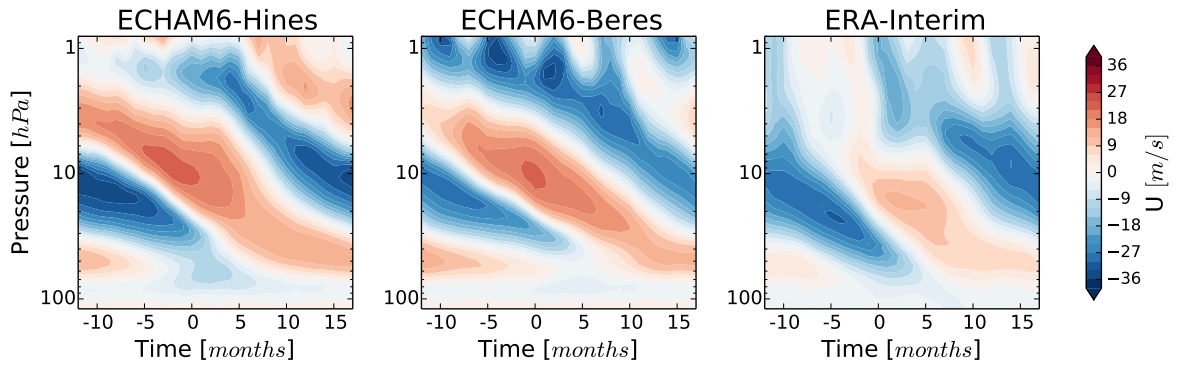
Figure 3.2: QBO composites of meridional ( 5^{\circ}\text{N} to 5^{\circ}\text{S} lat) and zonal mean zonal wind. Criterion for the composite is the onset of the westerly jet at 20\text{ hPa} . Comparison of the gravity wave parameterization with constant sources (ECHAM6-Hines) with the convection based gravity wave parameterization (ECHAM6-Beres) and reanalysis (ERA-Interim).
