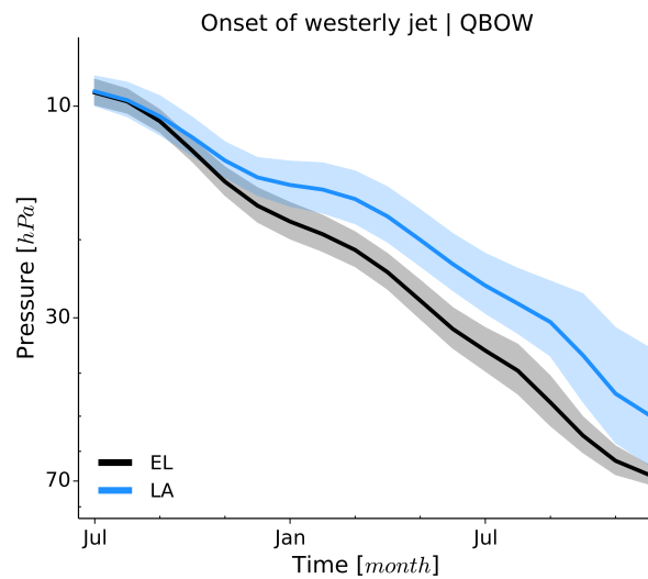
Figure 4.7: Timeseries of the onset of the westerly jet in QBOW for El Niño (black) and La Niña (blue) conditions. Solid lines show the ensemble means and shading indicates the range of two standard deviations ( 2\sigma ).
