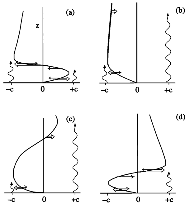
Figure 1.2: The QBO mechanism. Schematic representation of the temporal evolution (a-d) of QBO jets (solid line), driven by vertically propagating waves (curved arrows). Vertical axis depicts height, horizontal axis depicts zonal wind and horizontal phase speed. Double arrows illustrate wave-driven acceleration of the QBO jets, single arrows depict acceleration due to viscosity. Waves break where their horizontal phase speed c is close to the value of the QBO jets, the background wind. Illustration from Plumb (1984); Baldwin et al. (2001).
