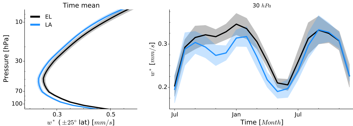
Figure 4.5: Upwelling w^* for El Niño (black) and La Niña (blue) conditions during QBOW phase. Upwelling w^* for QBOE phase (not shown) is qualitatively similar to QBOW phase. Zonal and meridional mean between -25^\circ and +25^\circ latitude. Solid lines show the ensemble means and shading indicates the range of two standard deviations ( 2\sigma ). Left panel: Vertical profile of time mean. Right panel: Timeseries at 30 \text{hPa} .
