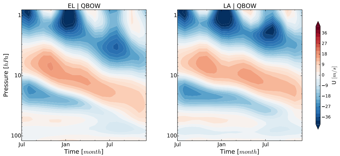
Figure 4.6: Evolution of the QBO for El Niño (left) and La Niña (right) conditions during QBOW phase. Timeseries of the profile of meridional and zonal mean zonal wind U for the ensemble mean.
