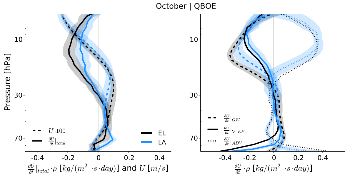
Figure 4.14: Same as figure 4.12, but for October of the first year instead of May of the second year.
