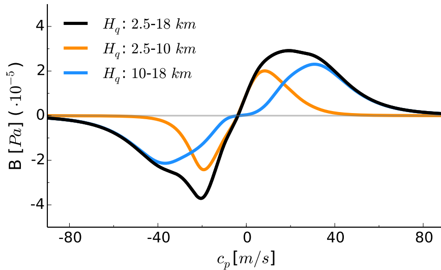
Figure 2.5: Separation of source spectrum into regimes of heating depth H_q . Zonal, meridional ( 5^\circ\text{N} to 5^\circ\text{S} lat) and time (5 years) mean source spectrum B for all cloud heating depths (black), shallow cloud heating depths (orange) and deep cloud heating depths (blue).
