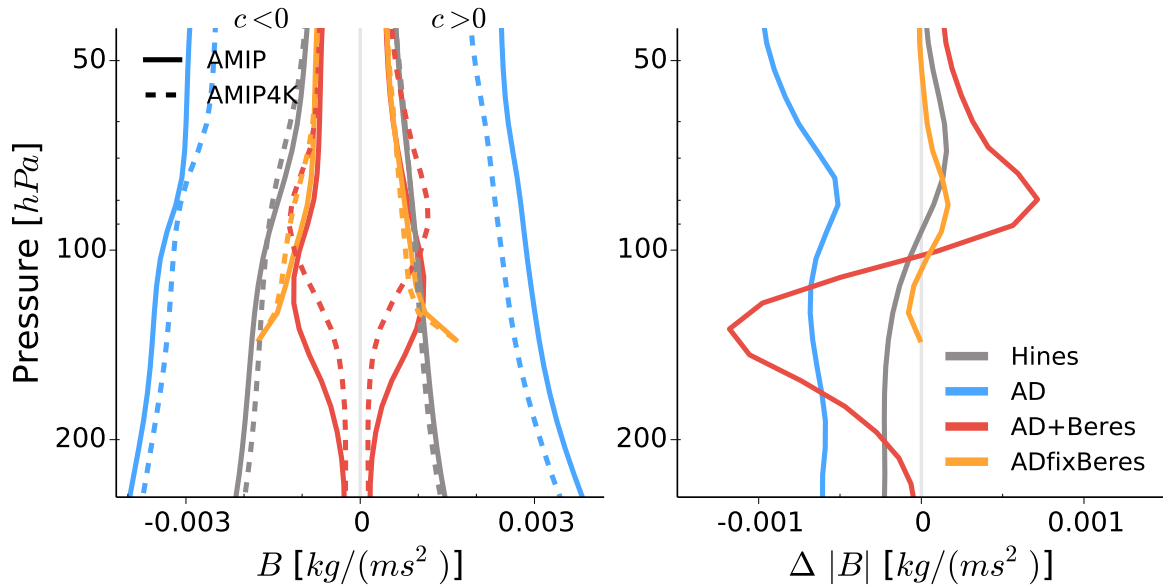
Figure 5.8: Vertical profile of gravity wave momentum flux ( B ) for the experiments Hines, AD, AD+Beres and ADfixBeres; time, zonal and meridional mean data. Left panel: B of easterly ( c < 0 ) and westerly ( c > 0 ) for present day (solid) and warmer climate (dashed). Right panel: Change of total momentum flux \Delta|B| = |B|_{AMIP4K} - |B|_{AMIP} , with |B| = |B_{c<0}| + |B_{c>0}| .
