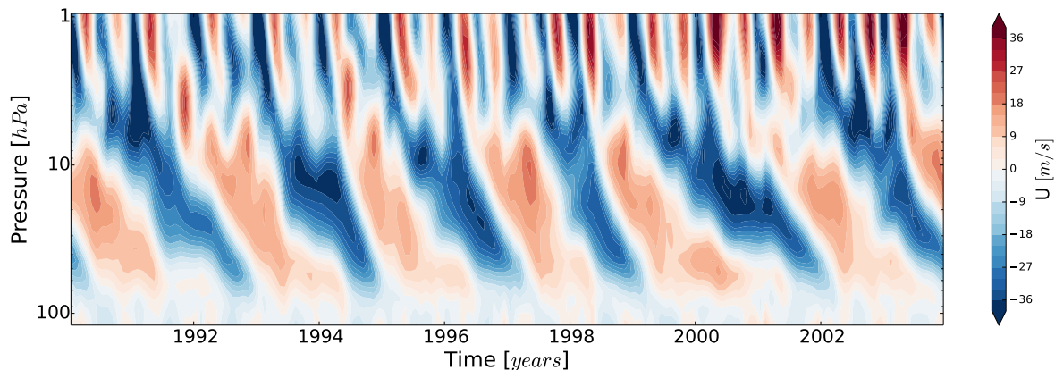
Figure 1.1: The QBO in ERA Interim. Timeseries of meridional ( 5^{\circ}\text{N} to 5^{\circ}\text{S} lat) and zonal mean zonal wind U in the stratosphere.
