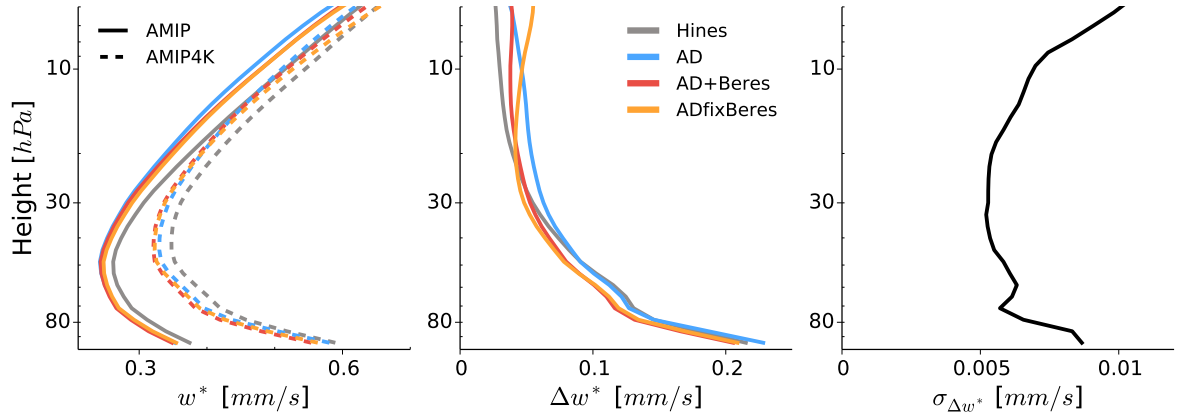
Figure 5.7: Vertical profile of residual vertical velocity w^* of a transformed Eulerian mean analysis for the experiments Hines, AD, AD+Beres and ADfixBeres; time, zonal and meridional ( \pm 25^\circ latitude) mean data. Left panel: w^* for present day (solid) and warmer climate (dashed). Center panel: Increase of w^* from present day climate to warmer climate, with \Delta w^* = w^*_{AMIP4K} - w^*_{AMIP} . Right Panel: Standard deviation \sigma of \Delta w^* of the four parameterization setups.
