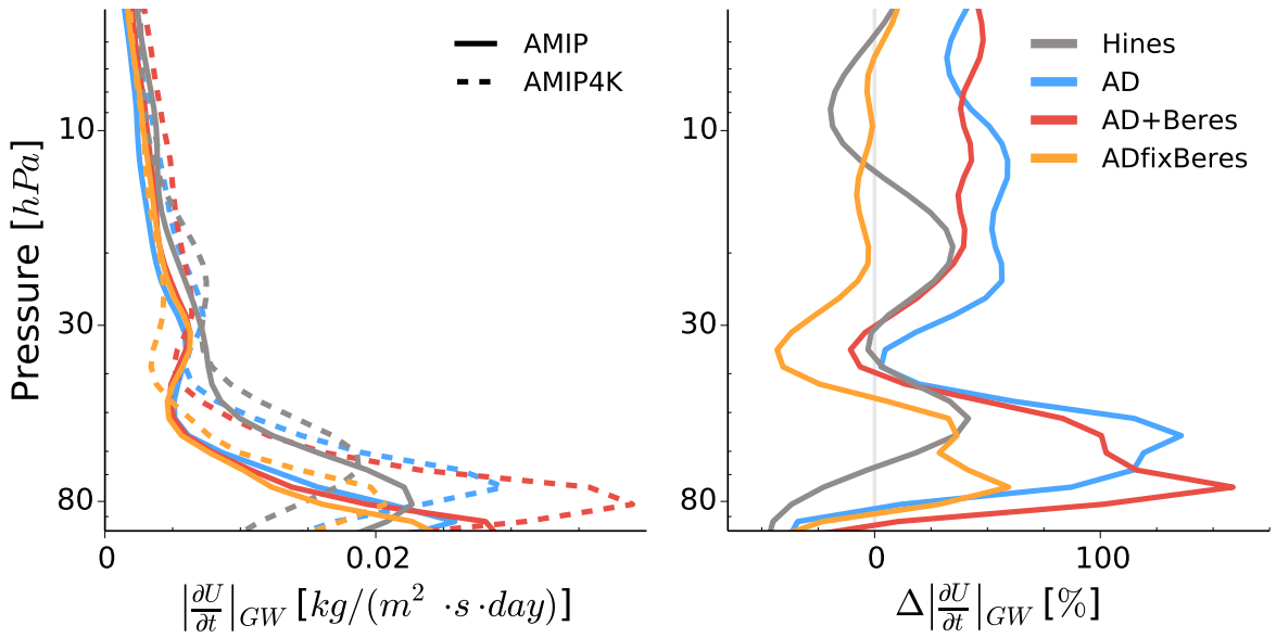
Figure 5.9: Vertical profile of zonal wind tendency due to gravity waves ( \frac{\partial U}{\partial t}|_{GW} ) for the experiments Hines, AD, AD+Beres and ADfixBeres; time, zonal and meridional mean data; \frac{\partial U}{\partial t} is scaled by density \rho . Left panel: Absolute tendency due to gravity waves with |\frac{\partial U}{\partial t}|_{GW} = |\frac{\partial U}{\partial t}|_{GW,c>0} + |\frac{\partial U}{\partial t}|_{GW,c<0} for present day (solid) and warmer climate (dashed). Right panel: Relative change of absolute tendency due to gravity waves \Delta |\frac{\partial U}{\partial t}|_{GW} .
