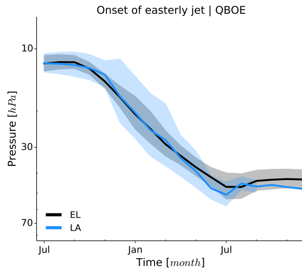
Figure 4.10: Timeseries of the onset of the easterly jet in QBOE for El Niño (black) and La Niña (blue) conditions. Solid lines show the ensemble means and shading indicates the range of two standard deviations ( 2\sigma ). Note that the ensemble consists of only one member during the last months of La Niña.
