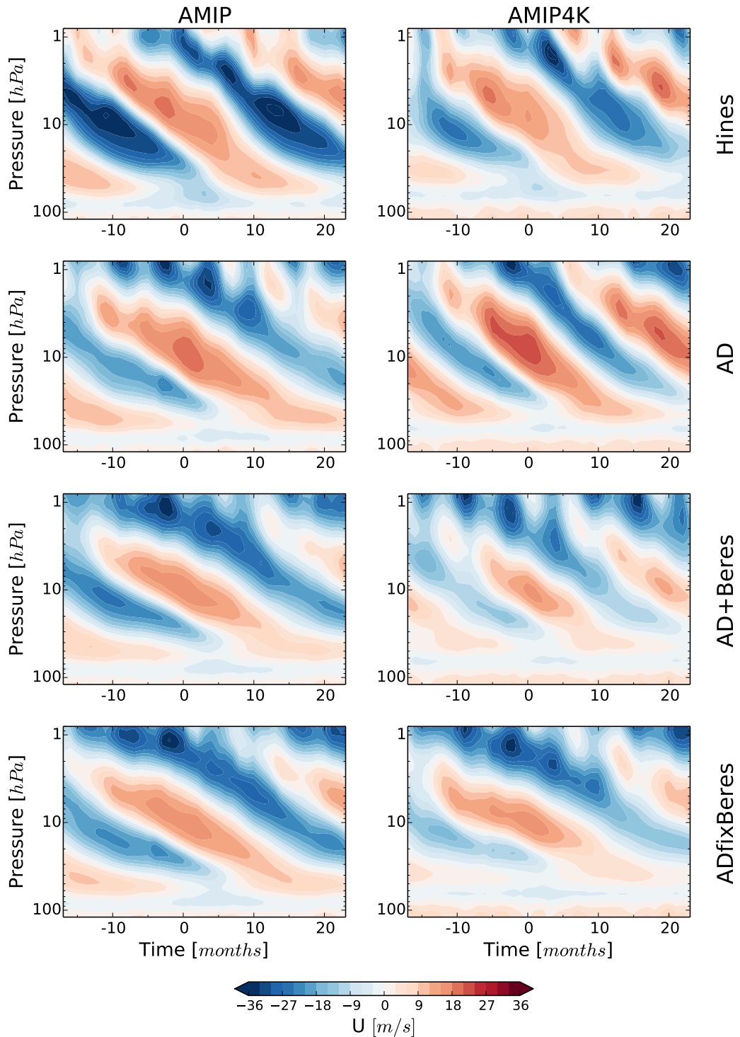
Figure 5.2: QBO composites for the experiments Hines, AD, AD+Beres and ADfixBeres, each for present day (left column) and warmer climate (right column). The onset of the westerly jet at 20 hPa is chosen as the criterion to calculate the composite, compiled from zonal and meridional mean zonal wind.
