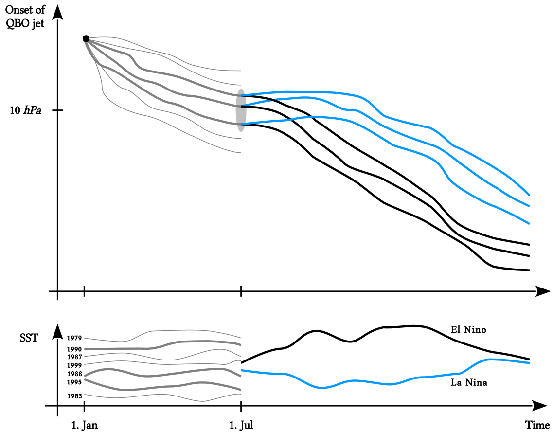
Figure 4.1: Illustration of the experimental setup. First part of the time axis until Jul 1 st shows the generation of an ensemble with similar QBO characteristics (thick gray), the second part of the time axis after Jul 1 st shows how the same ensemble reacts differently to El Niño (black) and La Niña (blue) conditions. The upper figure shows the position of the onset of the QBO jet, valid for both an easterly and a westerly jet, the lower figure illustrates the different SSTs to generate the ensemble and the different SSTs during El Niño and La Niña. The actual ensemble comprises 10 members, not three as illustrated in the figure and the actual number of model runs from which the ensemble is drawn is 30, not seven as illustrated in the figure.
