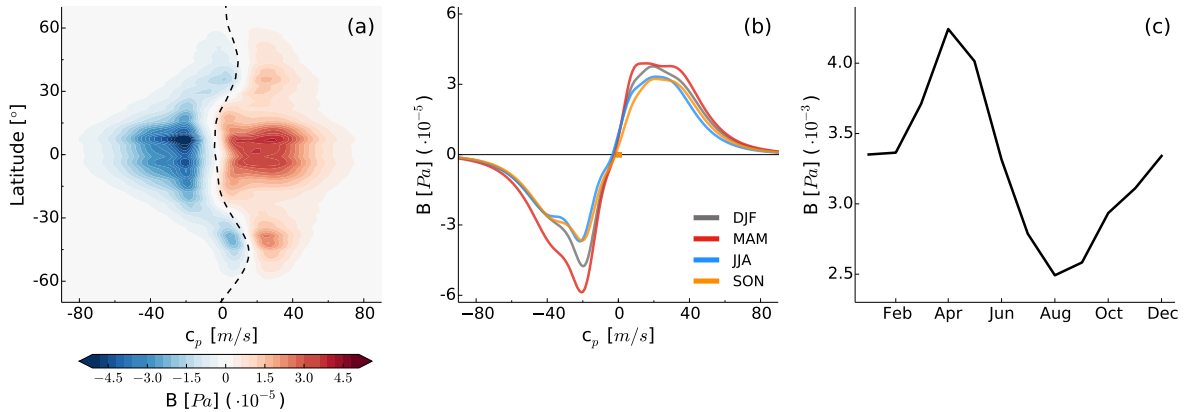
Figure 2.2: Source spectrum B of zonal momentum flux and its seasonal variability. (a) Latitudinal distribution of time and zonal mean source momentum flux as a function of phase speed. The dashed black line shows the zonal mean wind at 700hPa, the basis for the Doppler shift of the spectrum. (b) Zonal and meridional ( 5^\circ\text{N} to 5^\circ\text{S} lat) mean source spectra of zonal momentum flux in the four seasons. (c) Annual cycle of total zonal momentum flux B , zonal and meridional ( 5^\circ\text{N} to 5^\circ\text{S} lat) mean integrated over phase speed. All time averages cover 30 years (a-c).
