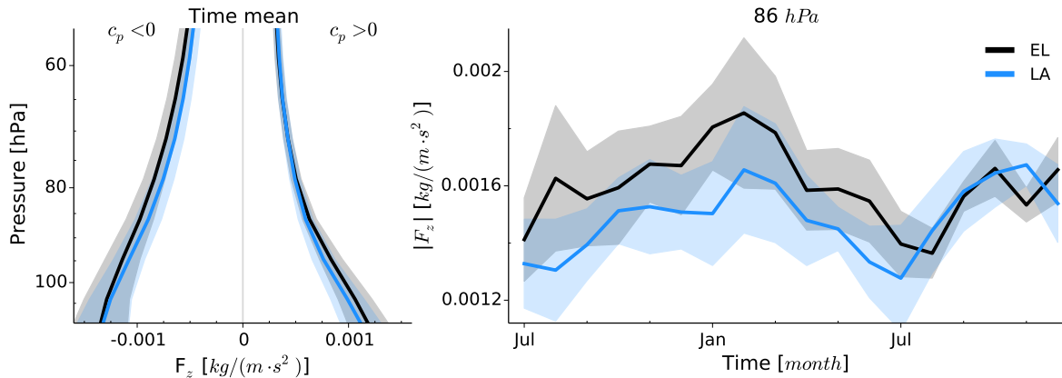
Figure 4.3: Vertical component F_z of the spectral EP-Flux vector for El Niño (black) and La Niña (blue) conditions during QBO phase. Vertical EP-Flux vector F_z for QBOE phase (not shown) is qualitatively similar to QBO phase. Zonal and meridional mean of F_z , scaled by density \rho , shows the integral over all frequencies and wave numbers. Solid lines show the ensemble means and shading indicates the range of two standard deviations ( 2\sigma ). Left panel: Vertical profile of time mean F_z for easterly ( c < 0 ) and westerly ( c > 0 ) waves. Right panel: Timeseries of absolute |F_z| at 86 hPa, with |F_z| = |F_{z,c<0}| + |F_{z,c>0}| .
