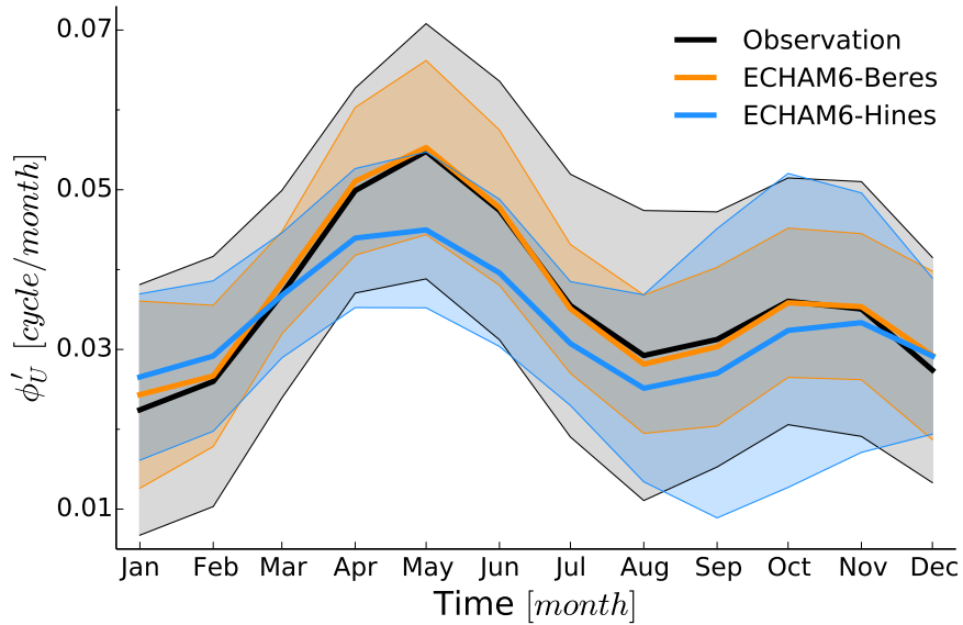
Figure 3.7: Sesaonal cycle of progression of qbo phases \phi' . The comparison with radiosonde observations from FU Berlin (black) shows an improvement of the convection based gravity wave parameterization in ECHAM6-Beres (orange) over ECHAM6-Hines with a gravity wave parameterization with constant sources (blue). Shaded areas show the 2\text{-}\sigma range.
