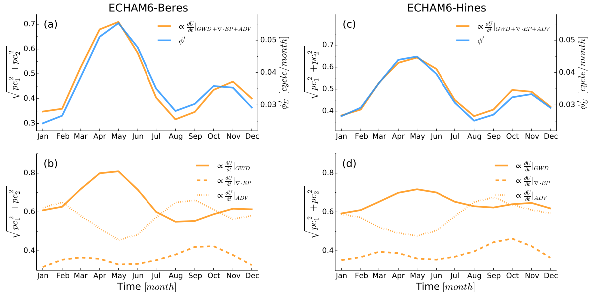
Figure 3.6: Seasonal cycle of progression of QBO phases (blue) and seasonal cycle of amount of zonal wind tendency (orange) for the Beres (a,b) and the Hines scheme (c,d). Comparison of qbo phase progression (blue) with amount of all tendency components (orange) for the Beres (a) and the Hines (c) scheme. Comparison of the individual tendency components of the entire tendency budget for the Beres (b) and the Hines (d) scheme. The drawn tendency is proportional to the actual tendency values, units are arbitrary. Note the two different y-axis in (a,c).
