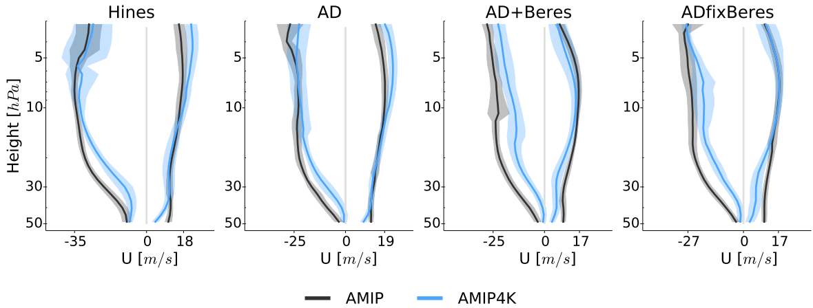
Figure 5.5: Vertical QBO amplitude profiles for the experiments Hines, AD, AD+Beres and ADfixBeres, each for present day (black) and warmer climate (blue), compiled from zonal and meridional mean zonal wind. The amplitude is calculated as the mean maximum wind speed of the QBO easterly ( U < 0 ) and westerly ( U > 0 ) jets on each vertical level. The shading illustrates the range of two standard deviations \sigma . The labels on the x-axis show the maximum value of the AMIP profiles.
