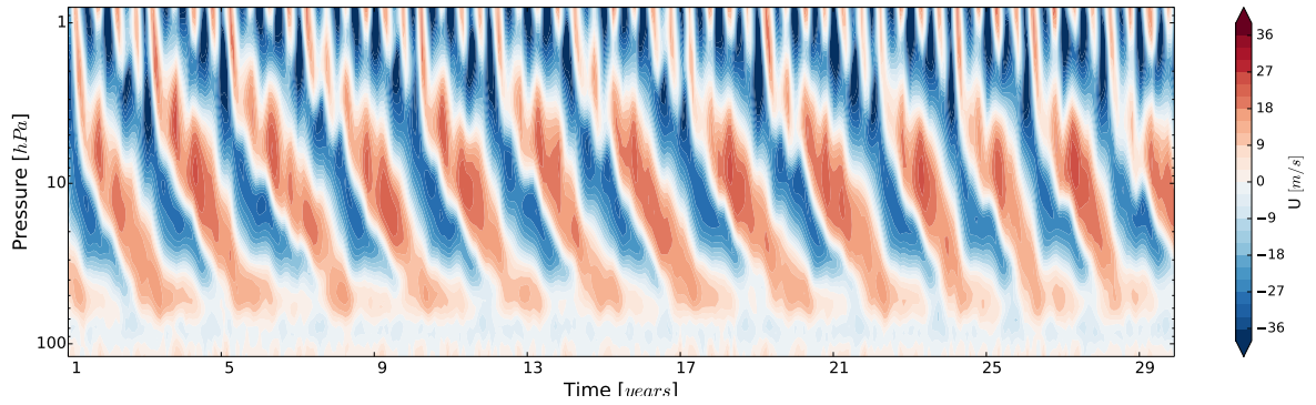
Figure 3.1: The QBO in ECHAM6-Beres. Timeseries of meridional ( 5^{\circ}\text{N} to 5^{\circ}\text{S} lat) and zonal mean zonal wind from a 30year model run with a purely convection based gravity wave source parameterization.
