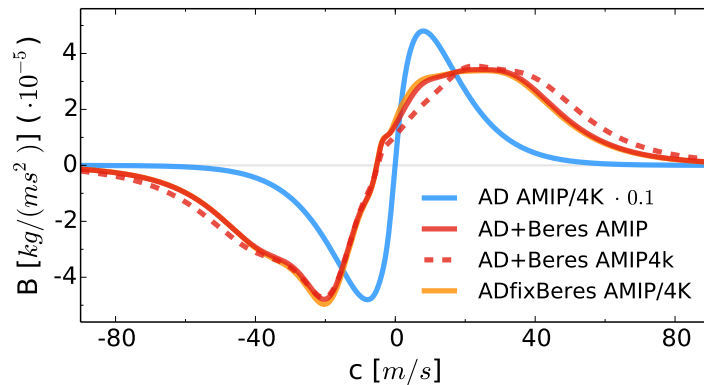
Figure 5.1: Momentum flux ( B ) source spectrum as a function of horizontal phase speed ( c ) for the experiments AD, AD+Berres and ADfixBerres; time, zonal and meridional mean. While the spectra of AD (blue) and ADfixBerres (orange) remain unchanged under AMIP and AMIP4K boundary conditions, the interactive source spectrum of AD+Berres (solid red) changes under the warmer climate of AMIP4K (dashed red). Note that the spectrum of AD is scaled by 0.1 for visualization reasons. ADfixBerres is hidden for the most part by AD+Berres AMIP.
