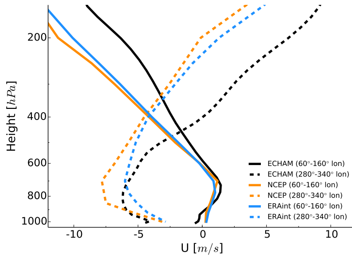
Figure 2.4: Zonal, meridional ( 5^{\circ}\text{N} to 5^{\circ}\text{S} lat) and time mean vertical wind profile for two regions, covering the eastern Indian ocean and Indonesia ( 60^{\circ} - 160^{\circ} lon, solid) and South America ( 280^{\circ} - 340^{\circ} lon, dashed). Comparison of ECHAM6-Beres simulation (black) with two reanalysis products: NCEP (orange) and ERA-Interim (blue). ECHAM6-Beres covers 30 years, NCEP 62 years and ERA-Interim 20 years.
