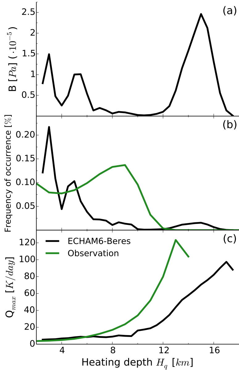
Figure 2.6: Influence of convection properties on the source momentum flux B (a) as a function of heating depth. Heating depth distribution (b) and maximum heating rate within a GCM grid box (c) (black) are compared to estimated observations (green) derived from geostationary infrared satellite data and TRMM.
