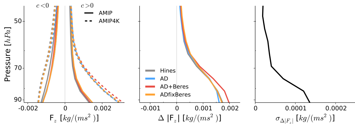
Figure 5.6: Vertical profile of vertical component F_z of the spectral EP-Flux vector for the experiments Hines, AD, AD+Beres and ADfixBeres; time (10years, based on 6 hourly data), zonal and meridional mean. F_z shows the integral over frequencies and wave numbers. Left panel: F_z of easterly ( c < 0 ) and westerly ( c > 0 ) waves for present day (solid) and warmer climate (dashed). Center panel: Change of the absolute value \Delta|F_z| = |F_z|_{AMIP4K} - |F_z|_{AMIP} from present day climate to the warmer climate, with |F_z| = |F_{z,c<0}| + |F_{z,c>0}| . Right Panel: Standard deviation \sigma of \Delta|F_z| of the four parameterization setups.
