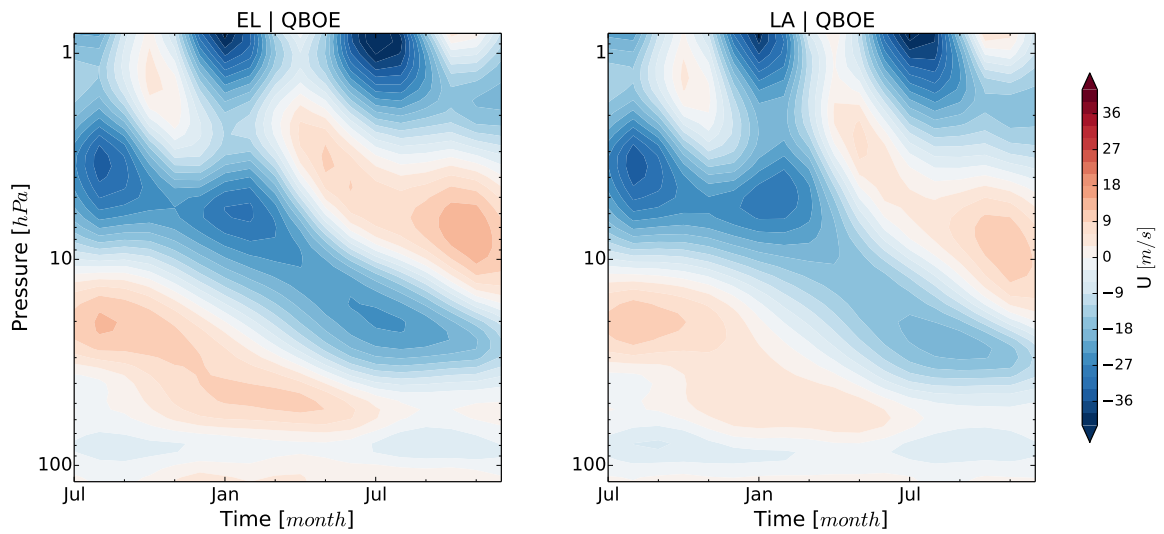
Figure 4.9: Evolution of the QBO for El Niño (left) and La Niña (right) conditions during QBOE phase. Timeseries of the profile of meridional and zonal mean zonal wind U for the ensemble mean.
