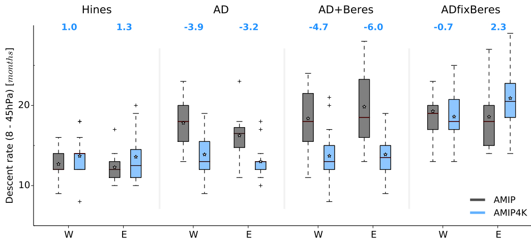
Figure 5.4: Distribution of QBO jet descent rates for the experiments Hines, AD, AD+Beres and ADfixBeres, each for present day (black) and warmer climate (blue), compiled from zonal and meridional mean zonal wind. The descent rate is determined for the westerly (W) and easterly (E) jet by calculating the time the wind maxima take from 8 hPa until 45 hPa . The difference (AMIP4K-AMIP) in the mean is drawn above. For details on box properties see figure 5.3.
