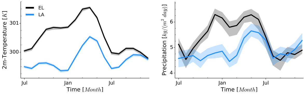
Figure 4.2: Timeseries of zonal and meridional mean temperature at 2 m (left) and precipitation (right) for El Niño (black) and La Niña (blue) conditions during QBOE phase. Temperature at 2 m and precipitation for QBOW phase (not shown) is qualitatively similar to QBOE phase. The shown precipitation is the total precipitation. Solid lines show the ensemble means and shading indicates the range of two standard deviations ( 2\sigma ).
