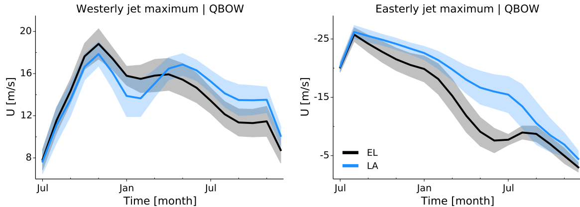
Figure 4.8: Timeseries of the strength of the westerly (left) and easterly (right) jet of QBOW for El Niño (black) and La Niña (blue) conditions. Solid lines show the ensemble means and shading indicates the range of two standard deviations ( 2\sigma ).
