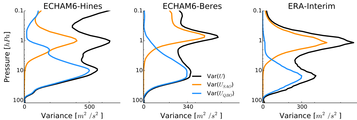
Figure 3.3: Variance over time (30 years) of meridional ( 5^{\circ}\text{N} to 5^{\circ}\text{S} lat) and zonal mean zonal wind. In order to compute the variance of the Semi-annual Oscillation \text{Var}(U_{SAO}) in orange and \text{Var}(U_{QBO}) in blue, a Fourier transform in time is applied to the winds, the periods between 5 and 7 months (SAO) and between 23 and 35 months (QBO) are selected to calculate each variance contribution. The variance over all periods \text{Var}(U) is depicted in black. Comparison of the gravity wave parameterization with constant sources (ECHAM6-Hines) with the convection based gravity wave parameterization (ECHAM6-Beres) and reanalysis (ERA-Interim). The label on the x-axis shows the maximum value of \text{Var}(U_{QBO}) .
