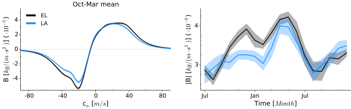
Figure 4.4: Gravity wave source momentum flux B for El Niño (black) and La Niña (blue) conditions during QBOE phase. Gravity wave source momentum flux B for QBOW phase (not shown) is qualitatively similar to QBOE phase. Zonal and meridional mean of B , scaled by density \rho , is determined at the top of convection. Solid lines show the ensemble means and shading indicates the range of two standard deviations ( 2\sigma ). Left panel: Source spectrum of B as a function of horizontal phasespeed c_p , time mean between October and March. Right panel: Timeseries of total amount of source momentum flux |B| integrated over c_p .
