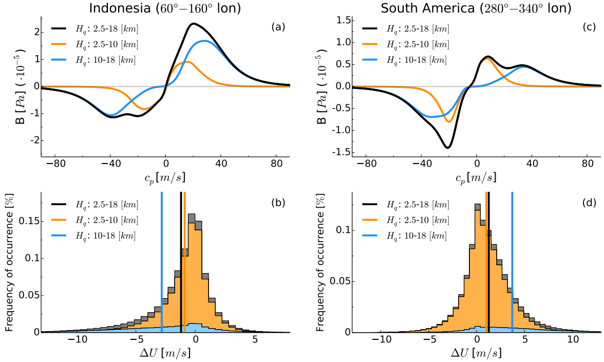
Figure 2.3: Effect of the background wind on the source spectrum, shown for two selected regions, centered over Indonesia ( 60^{\circ} - 160^{\circ} lon) (a,b) and over South America ( 280^{\circ} - 340^{\circ} lon) (c,d). Colors illustrate different regimes of heating depth: contribution from shallow heating depths (2.5 - 10 km, orange) and from deep heating depths (10 - 18 km, blue) to the entire range (2.5 - 18 km, black). Zonal, meridional ( 5^{\circ} N to 5^{\circ} S lat) and time (5 years) mean source spectra of zonal momentum flux (a,c). The spectral asymmetry is caused by wind shear, approximated as the mean wind relative to the zonal wind at 700 hPa \Delta U , within the vertical extent of the heating. The histogram of \Delta U is shown for different regimes of cloud heating depths (b,d) while the vertical lines denote the distribution mean.
