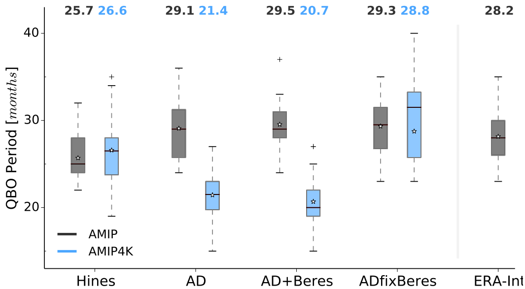
Figure 5.3: Distribution of QBO periods for the experiments Hines, AD, AD+Beres and ADfixBeres, each for present day (black) and warmer climate (blue), and the reanalysis ERA-Interim for present day climate. Periods are determined at the onset of the westerly jet at 20 hPa , compiled from zonal and meridional mean zonal wind. The distribution median is depicted by the horizontal line within each box, the distribution mean by the star whose value is drawn above. The box covers the interquartile range, distribution outliers are denoted by +.
