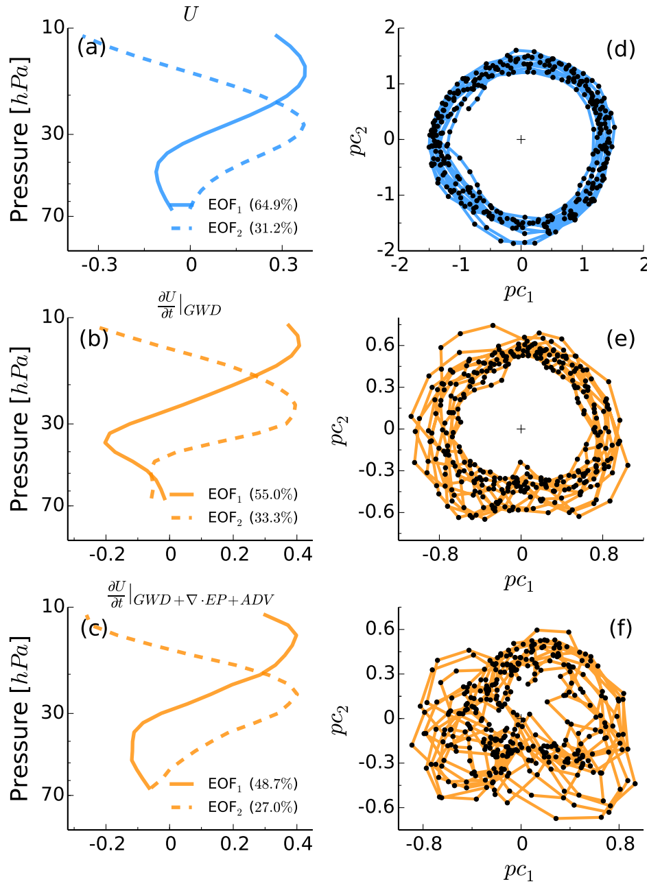
Figure 3.5: Empirical orthogonal functions ( EOF ) (a)-(c) and principal components ( pc ) (d)-(f) of zonal wind U (a,d), tendency of zonal wind due to gravity waves \frac{\partial U}{\partial t}|_{GW} (b,e) and the total tendency of all components \frac{\partial U}{\partial t}|_{GW + \nabla \cdot EP + ADV} (c,f). The numbers in the legend (a)-(c) indicate the fraction of variance that each EOF accounts for. The pcs in (d) are scaled to unit variance, units on individual plots are arbitrary. The EOFs and pcs of \frac{\partial U}{\partial t}|_{\nabla \cdot EP} and \frac{\partial U}{\partial t}|_{ADV} are not shown individually; they are qualitatively similar to \frac{\partial U}{\partial t}|_{GWC} in (b,e).
