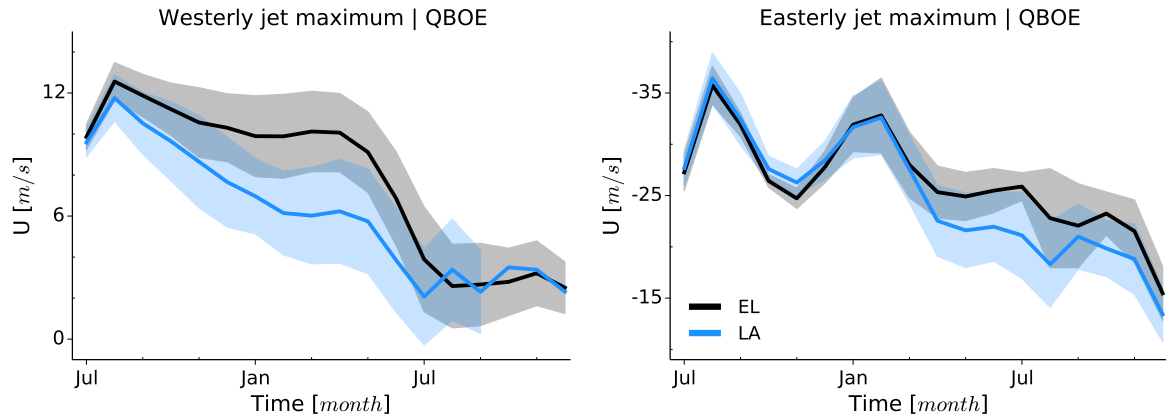
Figure 4.11: Timeseries of the strength of the westerly (left) and easterly (right) jet of QBOE for El Niño (black) and La Niña (blue) conditions. Solid lines show the ensemble means and shading indicates the range of two standard deviations ( 2\sigma ). Note that the ensemble for the westerly jet consists of only one member during the last months of La Niña.
