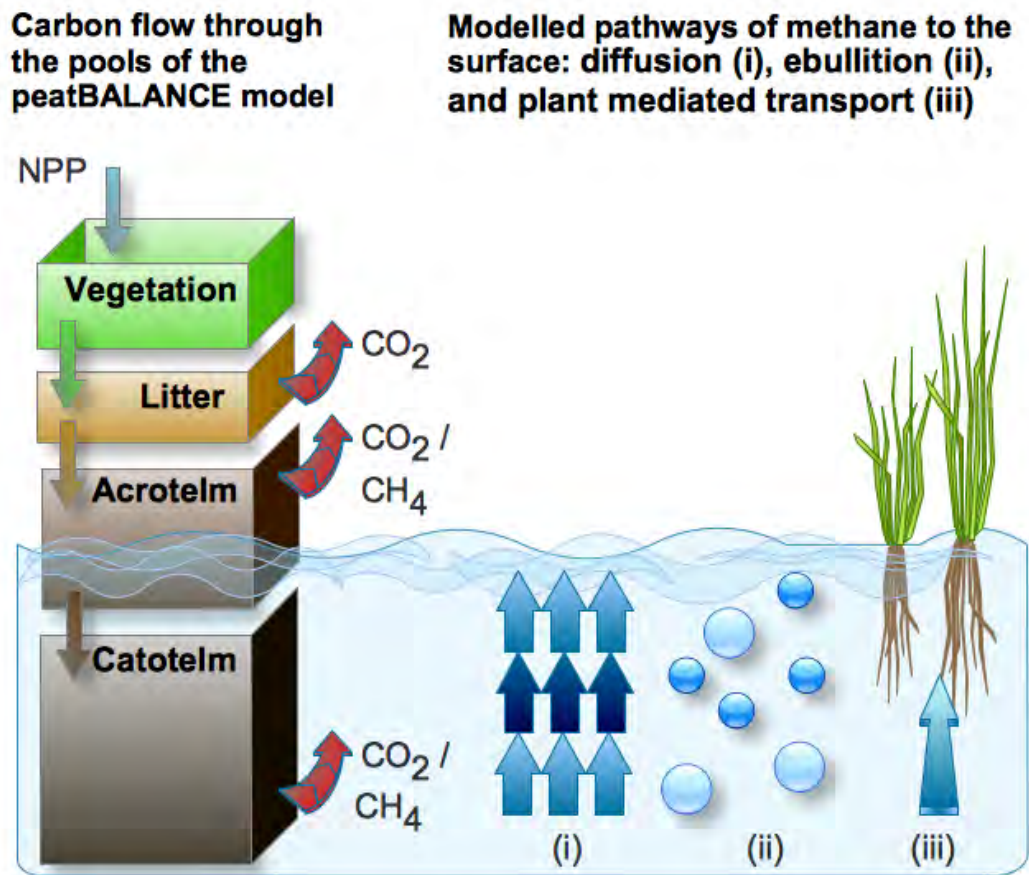
Figure 1: Diagrammatic sketch of the carbon fluxes in the peatBALANCE model. The transport pathways of \text{CH}_4 fluxes are shown at the right.
