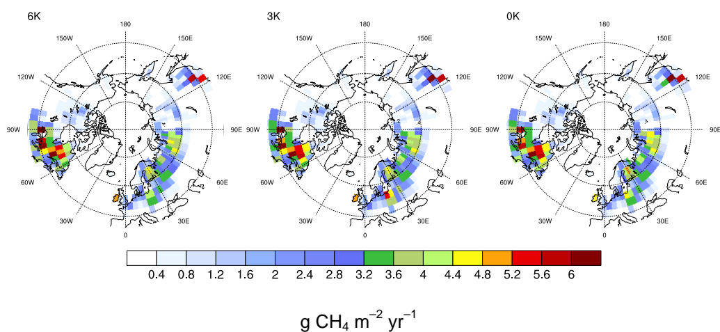
Figure 7: Methane emissions ( \text{g CH}_4 \text{ m}^{-2} \text{ yr}^{-1} ) from the time slice simulations for 6000 yr BP (left), 3000 yr BP (middle) and pre-industrial (right), averaged over 10 yr of model simulation. Carbon fluxes are represented with respect to grid box area.
