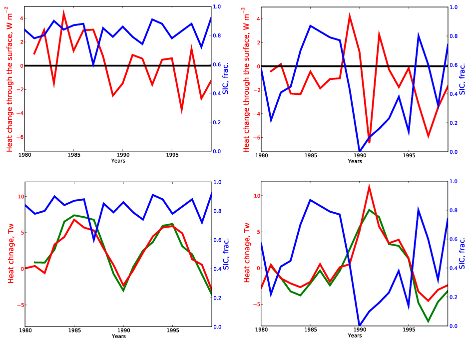
Figure 2.16 — Top:Heat change through the surface (red) and September SIC (blue). Bottom: heat convergence (red), total heat content change (green) and September SIC(blue). Left: ECHAM run, right: FNCEP run.
