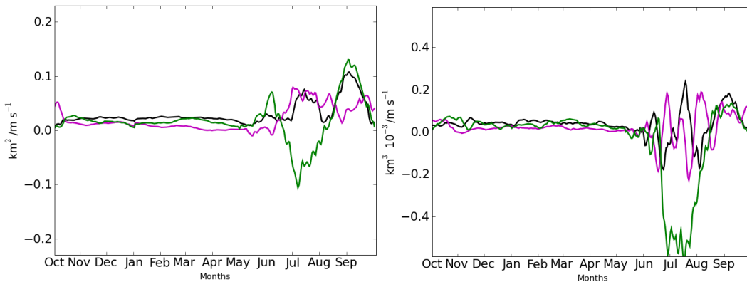
Figure 3.33 — Evolution of the mean daily AREA (left) and VOLUME (right) sensitivities to the V wind component in Box 4. Black: 1980-1989; magenta: 1990-1999; green: 2000-2007.
