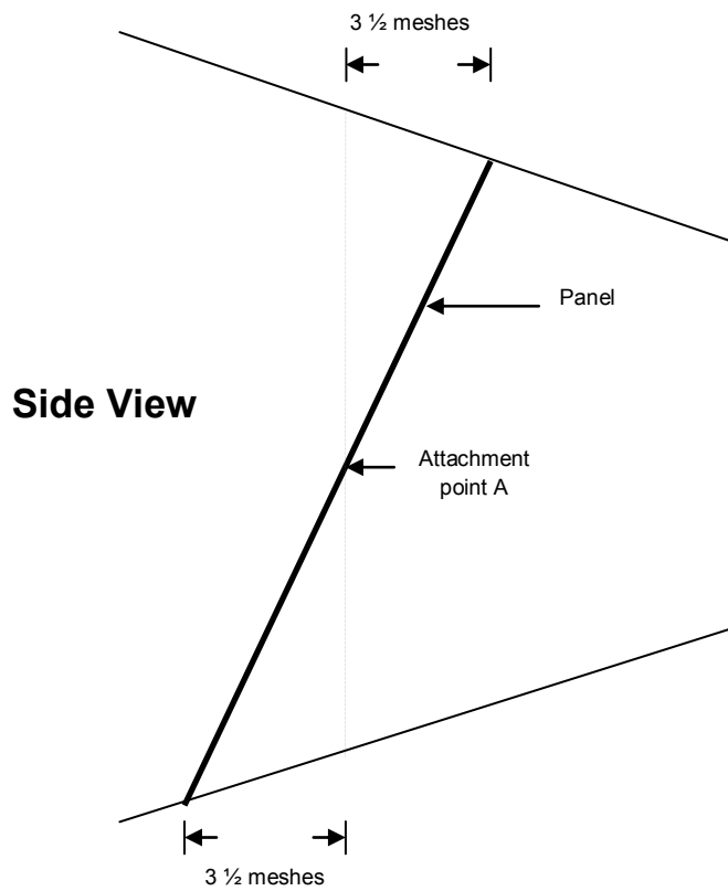
Figure 3: Side view of position of the Faithlie Cod Avoidance Panels (FCAP and FCAP2).
