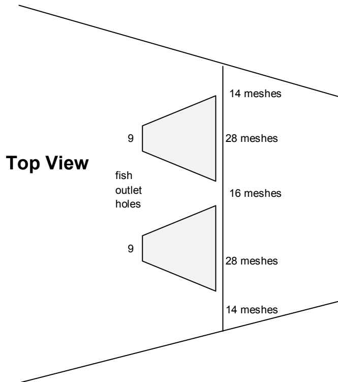
Figure 5: Top view of design and position of fish outlet holes of the modified Faithlie Cod Avoidance Panel (FCAP2).
