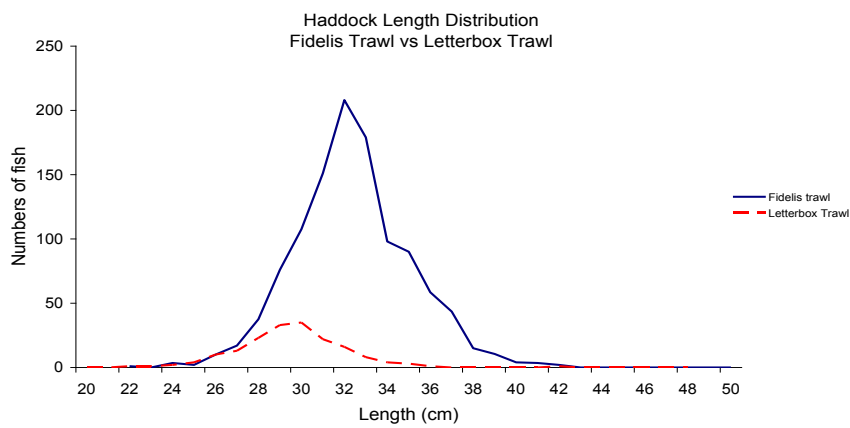
Figure 10: Haddock length distribution for Fidelis and Letterbox trawls.
