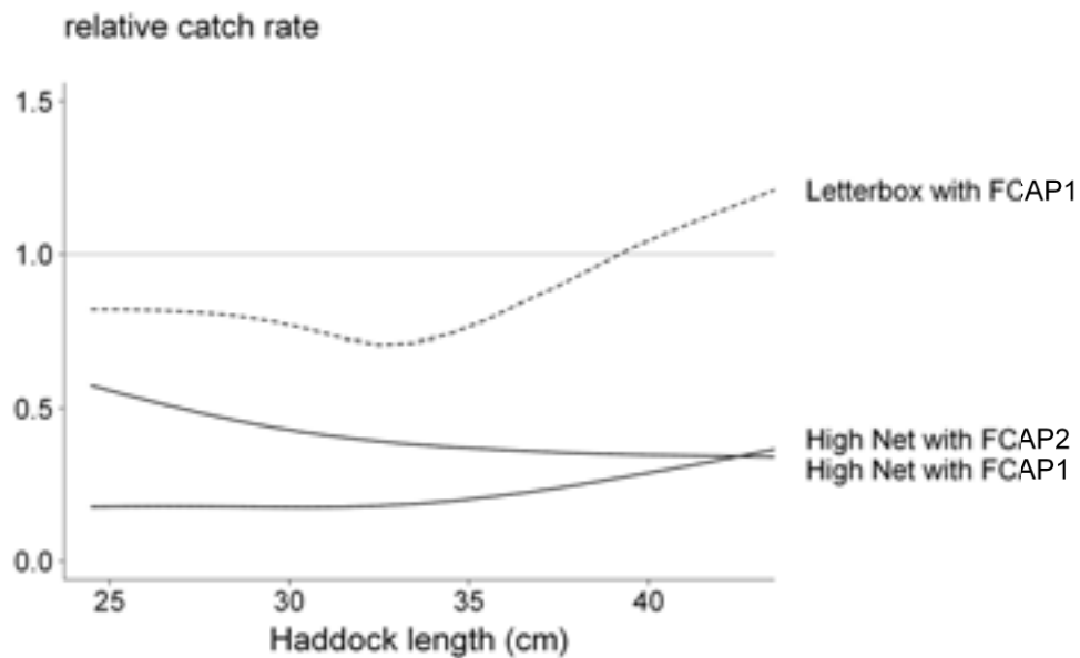
Figure 7: The selective performance of the Fidelis trawl with (i) the FCAP1 fitted; and (ii) the FCAP2 fitted, in relation to a standard Fidelis trawl; and the selective performance of the Letterbox trawl with the FCAP1 fitted in relation to a standard Letterbox trawl.
