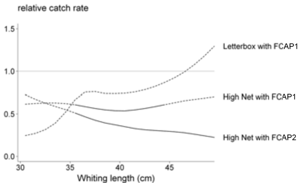
Figure 8: The selective performance of the Fidelis trawl with (i) the FCAP1 fitted; and (ii) the FCAP2 fitted, in relation to a standard Fidelis trawl; and the selective performance of the Letterbox trawl with the FCAP1 fitted in relation to a standard Letterbox trawl.
