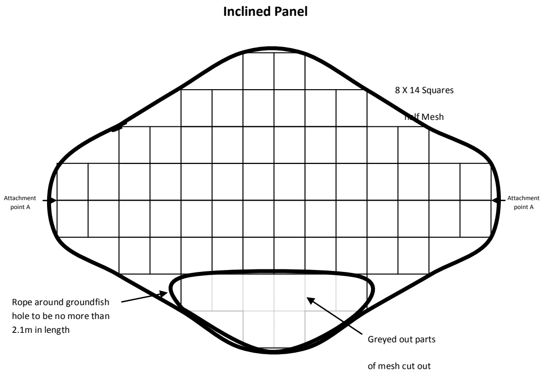
Figure 1: Design of inclined panel.
