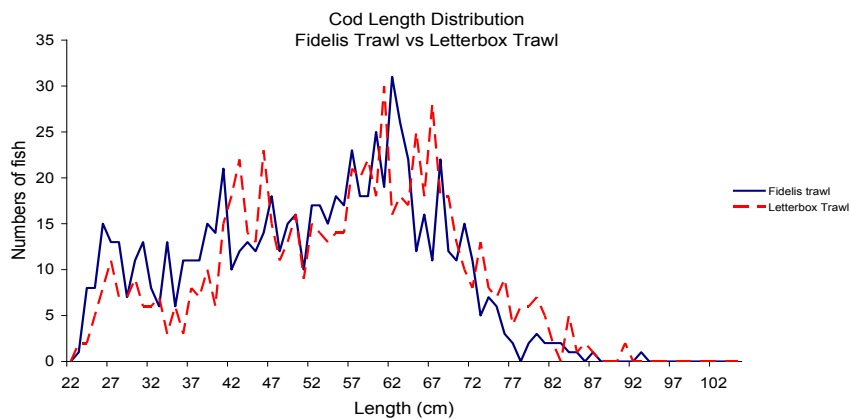
Figure 9: Cod length distribution for Fidelis and Letterbox trawls.
