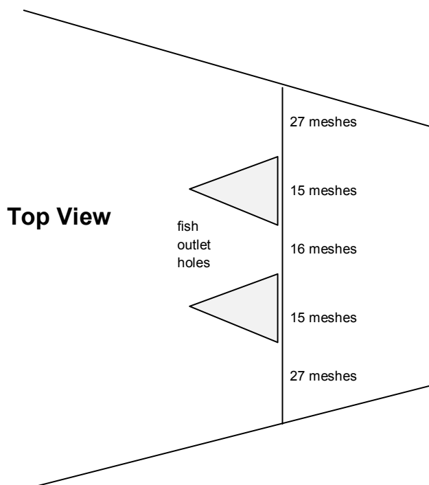
Figure 4: Top view of design and position of fish outlet holes of the original Faithlie Cod Avoidance Panel (FCAP).
