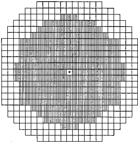
Fig. 2a FCAL front view
