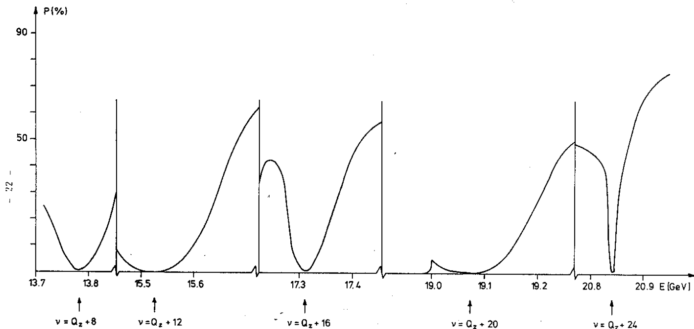
Fig. 7 Depolarizing Resonances \nu = Q_z + 4n for PETRA in the energy region 13 - 21 GeV
