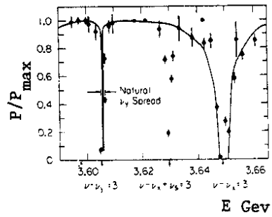
Fig. 3c. Detail of SPEAR polarization curve showing non-linear resonance: a\delta - Q_x + Q_s = 3 (From Ref. 11)
