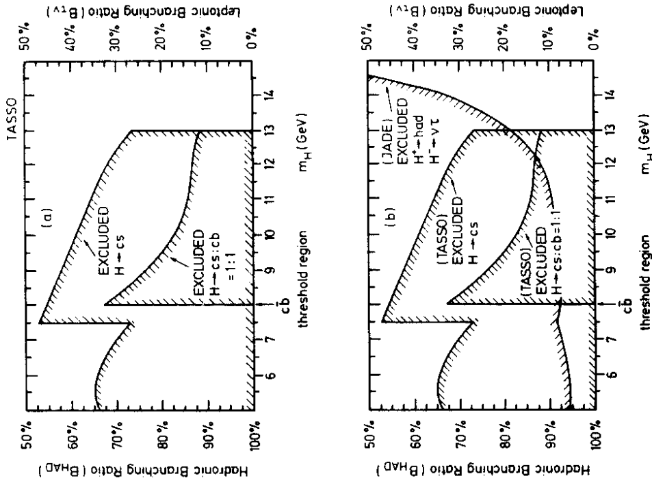
Fig. 41 - (a) : Limits on the hadronic branching ratio ( B_{had} ) as a function of H^\pm mass from this experiment
