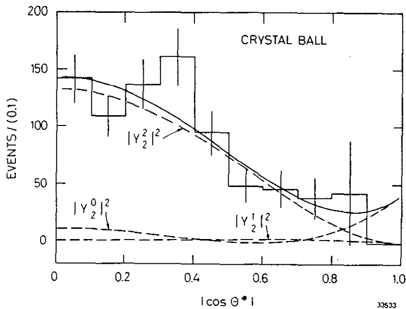
Fig. 8.4 - The decay angular distribution of f^0 \rightarrow \pi^0 \pi^0 . The data - corrected for the acceptance - are from the Crystal Ball Collaboration.
