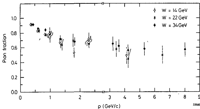
Fig. 6.11 - The pion fraction in e^+e^- \rightarrow \text{hadrons} as a function of momentum for various c.m. energies. The data are from the TASSO Collaboration.
