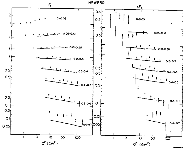
Fig. 9.18 - The structure functions F_2 and xF_3 as measured by the HPWFRO Collaboration. Curves correspond to a fit to the CHARM data.
