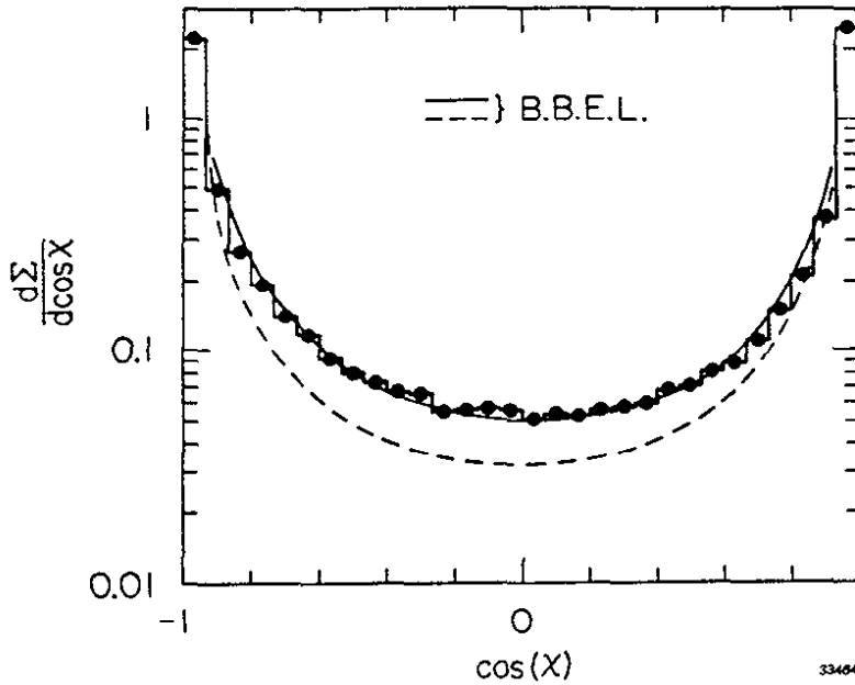
Fig. 7.29 - The angular dependence of the energy-energy correlation function. The dashed curve shows the parton level QCD prediction, the solid line includes hadronization effects. The data are from the MARK II Collaboration.
