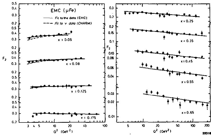
Fig. 9.19 - The structure function F_2 as measured by the EMC. The dashed curves correspond to a fit to the CHARM data only. Where the fit to the EMC data (full lines) agrees with the CHARM fit only a full line is drawn).
