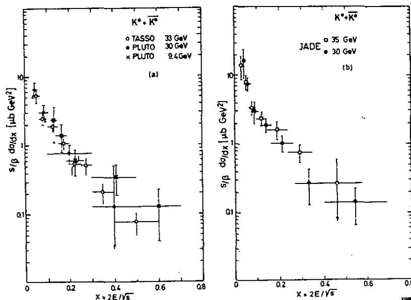
Fig. 6.13 - The invariant cross section s/\beta \, d\sigma/dx for inclusive K^0 + \bar{K}^0 production versus x for various c.m. energies.
