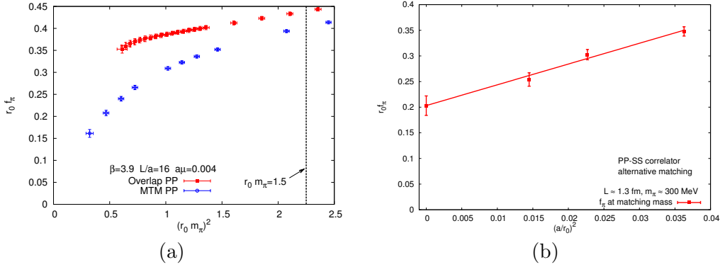
Fig. 5. (a) Matching of overlap and MTM quark masses (ensemble B_{\ell, V_1} ) at a heavy quark mass value (yielding r_0 m_\pi = 1.5 , which is denoted by vertical line), where the zero modes effects are strongly suppressed. Idea of the matching is explained in the text. (b) Continuum limit of f_\pi in the case of the alternative matching condition.
