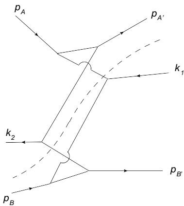
FIG. 3: The 3 \rightarrow 3 gluon scattering amplitude with discontinuity in t_2 channel.
