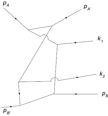
FIG. 4: The 3 \rightarrow 3 gluon scattering amplitude for the Mandelstam channel, where t_2, s, s_1, s_3 < 0 and s_{13}, s_{02} > 0 .
