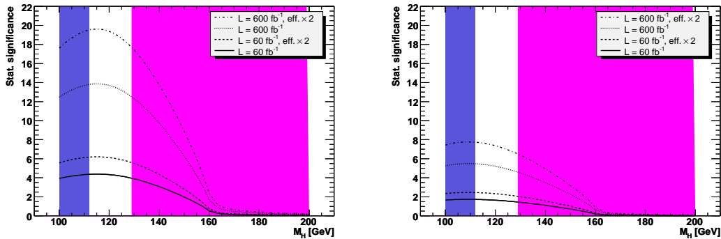
Figure 1: Significances reachable CED Higgs production in the SM4 in the H \rightarrow b\bar{b} (left plot) and H \rightarrow \tau^+\tau^- (right plot) channel for effective luminosities of “60 fb -1 ”, “60 fb -1 eff×2”, “600 fb -1 ” and “600 fb -1 eff×2”. The regions excluded by LEP appear as blue/light grey for low values of M_{H^{\text{SM4}}} and excluded by the Tevatron as red/dark grey for larger values of M_{H^{\text{SM4}}} .
