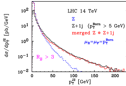
Figure 2: The p_T distribution of the next-to-hardest jet in single Z production (blue dashed curve), in Z + 1 \text{ jet} (black solid) and in the merged sample (red solid).
