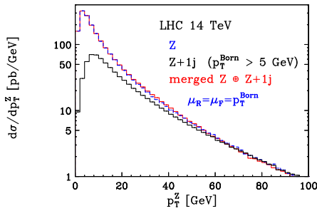
Figure 1: The p_T distribution of the Z boson in single Z production (blue dashed curve), in Z + 1 \text{ jet} (black solid) and in the merged sample (red solid).
