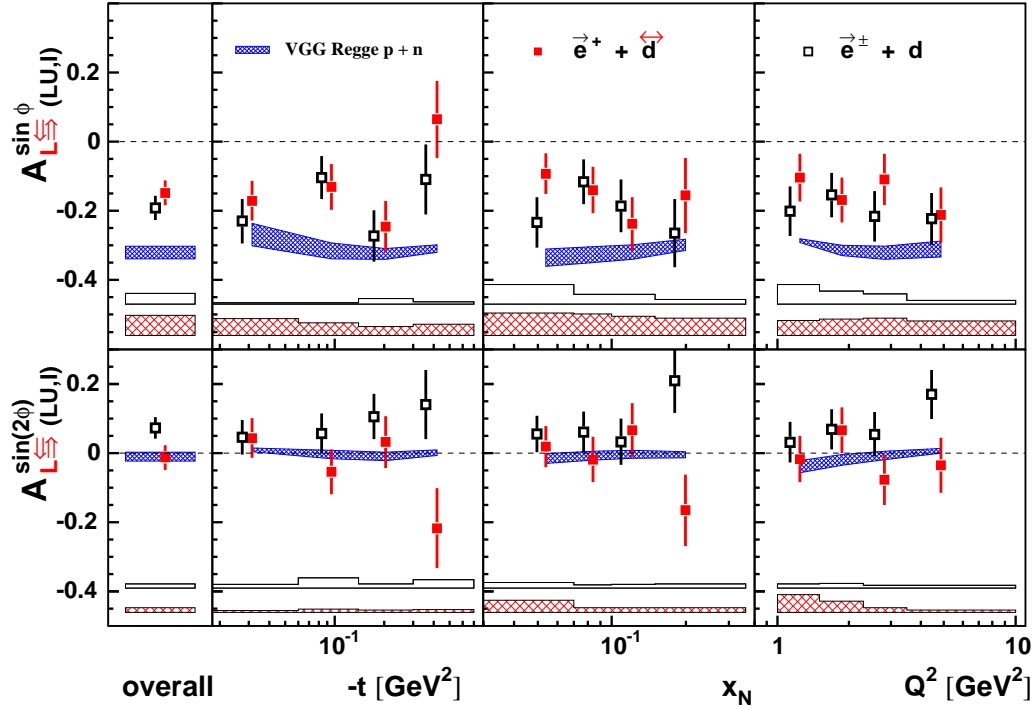
Fig. 1. Results from the present work (red filled squares) representing single-charge beam-helicity asymmetry amplitudes A_{L, \pm}^{\sin(n\phi)} describing the dependence of the sum of squared DVCS and interference terms on the beam helicity, for a tensor polarization of P_{zz} = 0.827 (indicated by the symbol \leftrightarrow ). The black open squares represent charge-difference amplitudes A_{L, \pm}^{\sin(n\phi)} from only the interference term, extracted from unpolarized deuterium data [27]. The error bars represent the statistical uncertainties, while the coarsely hatched (open) bands represent the systematic uncertainties of the filled (open) squares. There is an additional overall 1.9% (2.4%) scale uncertainty arising from the uncertainty in the measurement of the beam polarization in the case of polarized (unpolarized) deuterium data. The points for unpolarized deuterium data are slightly shifted to the left for better visibility. The finely hatched band shows the results of theoretical calculations for the combination of incoherent scattering on proton and neutron, using variants of the VGG double-distribution model [45,48] with a Regge ansatz for modeling the t dependence of GPDs [49].
