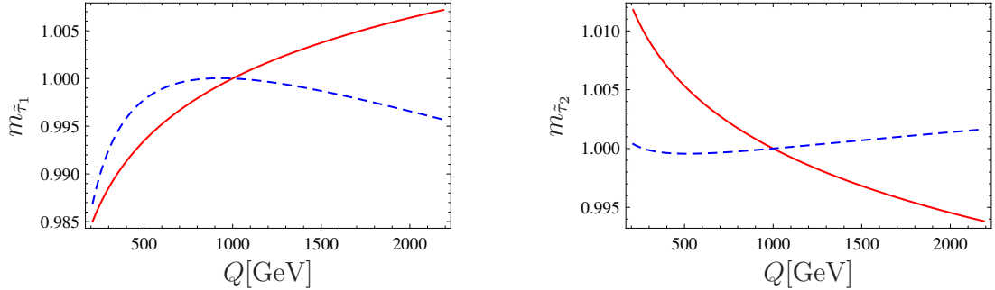
Figure 4: Dependence of the stau masses of the sleptons on the renormalization scale Q at tree (red) and 1-loop level (dashed blue) normalized to the value at Q = 1 TeV.
