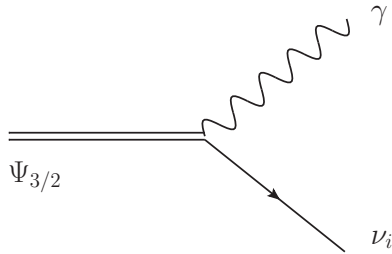
Figure 2: Gravitino decay into photon and neutrino.
