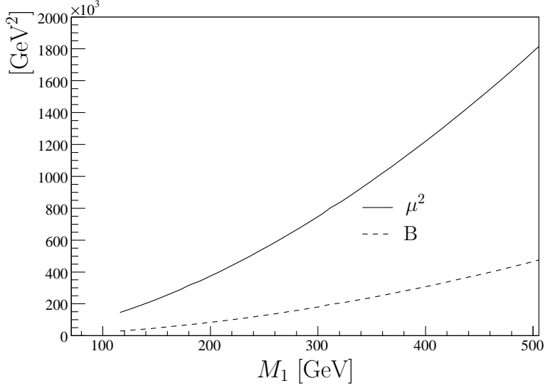
Figure 1: The parameters \mu and B of Eqs. (3) and (4), respectively, as functions of the bino mass M_1 . The plot has been obtained by means of SOFTSUSY3.0 [23].
