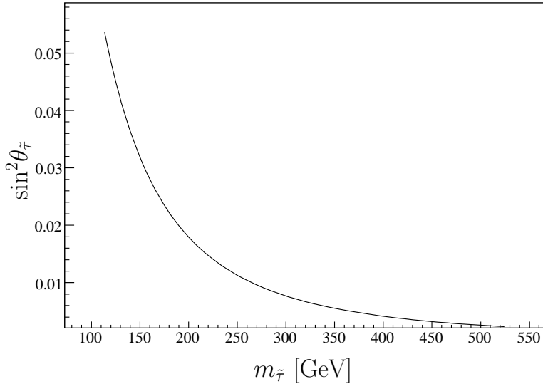
Figure 5: \tilde{\tau} -mixing angle: \sin^2(\theta_\tau) as function of the lightest \tilde{\tau} -mass m_{\tilde{\tau}_1} .
