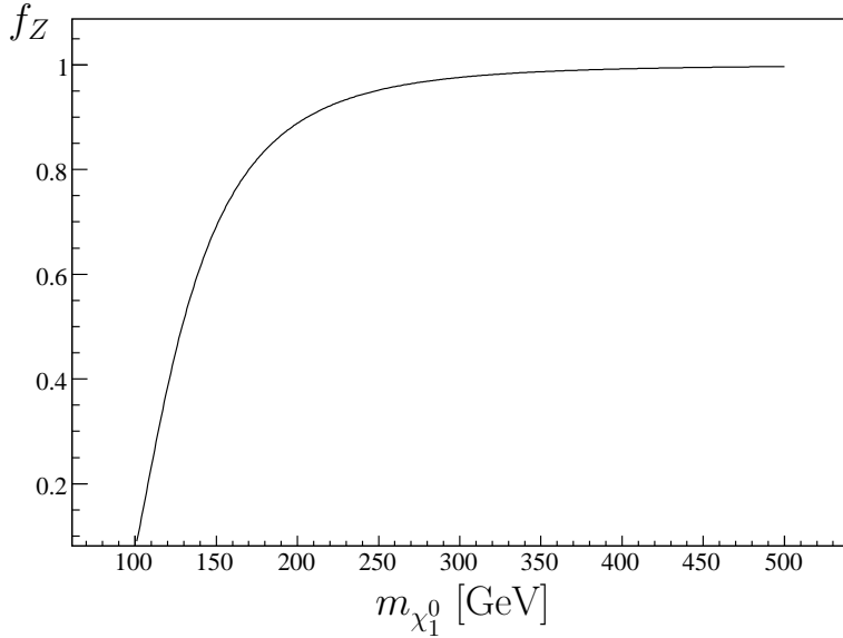
Figure 4: Phase space suppression factor for neutralino decay to Z-boson and neutrino.
