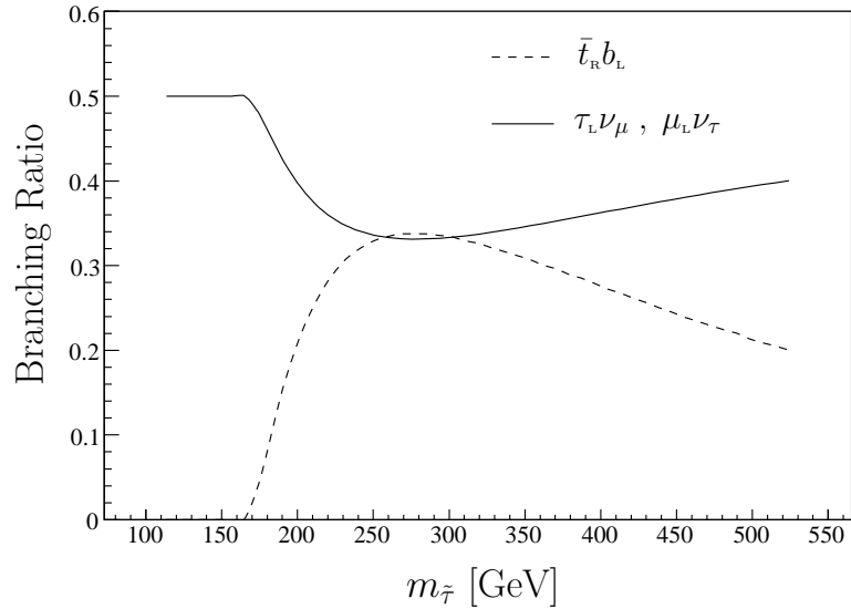
Figure 7: \tilde{\tau}_1 -branching ratios as functions of m_{\tilde{\tau}_1} . The dependence on the \tilde{\tau}_1 -mass is determined by the top-bottom threshold and the mass dependence of the \tilde{\tau}_1 -mixing angle.
