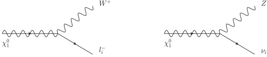
Figure 3: Neutralino decays into charged lepton and W-boson, and neutrino and Z-boson.
