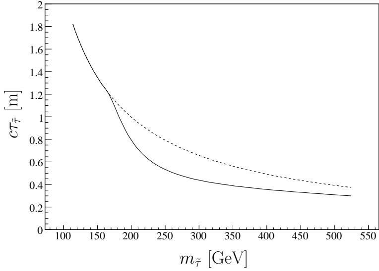
Figure 6: \tilde{\tau}_1 -decay length as function of m_{\tilde{\tau}_1} . Above the top-bottom threshold hadronic decays decrease the \tilde{\tau}_1 -lifetime.
