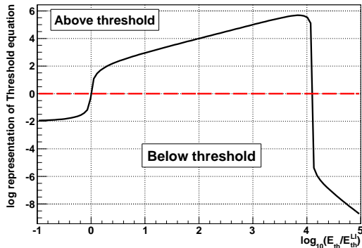
FIG. 1. Equation (7) is drawn for \xi/2 + \xi_I = 10^{-12} . On the y -axis \text{sign}(\text{Eq. (7)}) \cdot \log_{10}(|\text{Eq. (7)}|/0.01) is drawn, where 0.01 is just a small value. Positive values on the y -axis mean that the reaction is allowed, while negative values mean that it is forbidden. Both lower and upper thresholds are present.
