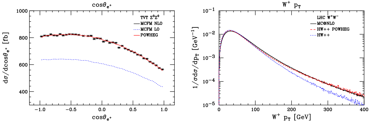
(a) Cosine of the polar angle of a positron produced from a decaying Z^0 boson, in its rest frame, in Z^0Z^0 pair production at the Tevatron ( \sqrt{s} = 1.96 TeV). The Herwig++ POWHEG prediction is shown in red while the NLO and LO predictions of MCFM appear as black stars and blue dots respectively.
