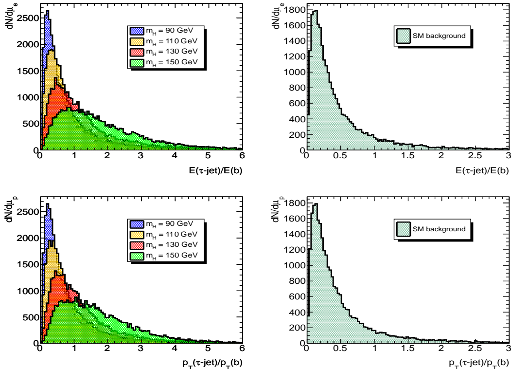
FIG. 6: Distributions in the ratio E(\tau\text{-jet})/E(b) and p_T(\tau\text{-jet})/p_T(b) from the process pp \rightarrow t\bar{t}X , followed by the decay t \rightarrow W^+b (right-hand frames), and the same distributions for the decay chain t \rightarrow H^+b with the four indicated charged Higgs masses (left-hand frame).
