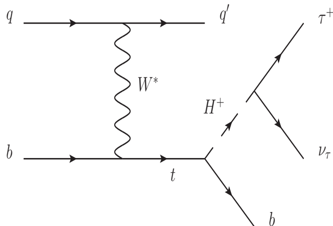
FIG. 10: Feynman diagram for qb \rightarrow q't , followed by the decay t \rightarrow b(H^+ \rightarrow \tau^+\nu_\tau) .
