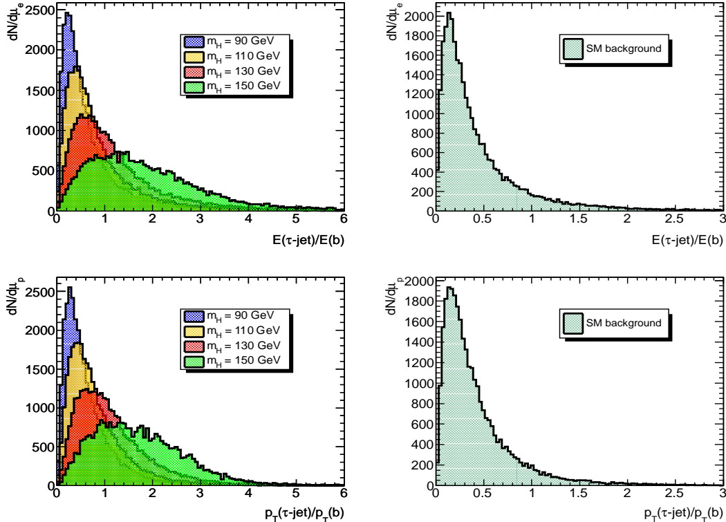
FIG. 14: Distributions in the ratio E(\tau - \text{jet})/E(b) and p_T(\tau - \text{jet})/p_T(b) from the process pp \rightarrow t/\bar{t}X , followed by the SM decay t \rightarrow W^+b (right-hand frames), and the same distributions for the decay chain t \rightarrow H^+b with the four indicated charged Higgs masses (left-hand frame).
