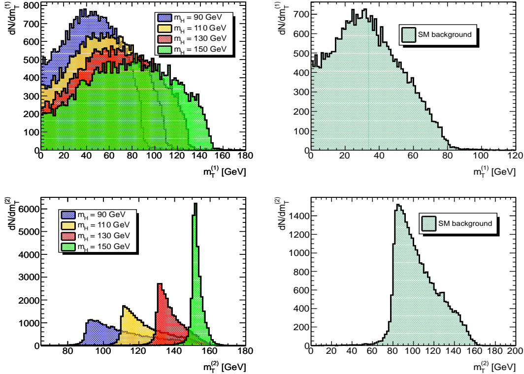
FIG. 16: Transverse mass distributions for the W^\pm in the process pp \rightarrow t/\bar{t} + X followed by the decay t \rightarrow bW^+ (right-hand frames) and for the H^\pm transverse mass for the decay chain t \rightarrow H^+b with the four indicated charged Higgs masses (left-hand frame). The definitions used for defining the transverse masses m_T^{(1)} and m_T^{(2)} are given in the text.
