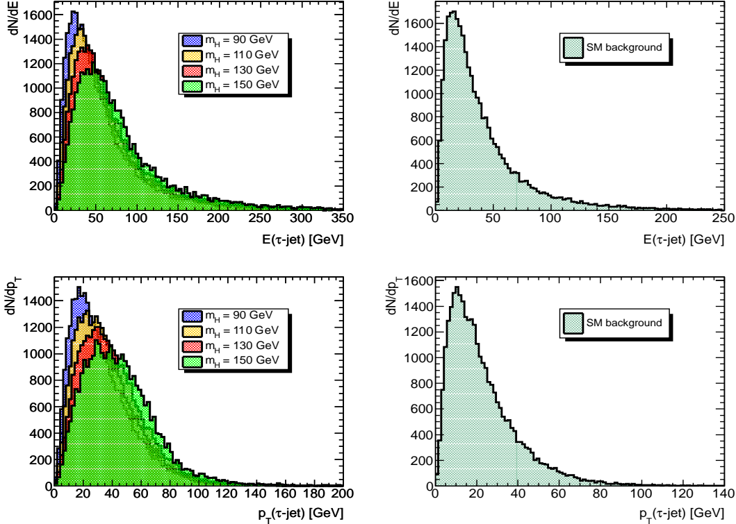
FIG. 13: Distributions in the energy of the \tau -jet, E(\tau - \text{jet}) , and transverse momentum of the \tau -jet, p_T(\tau - \text{jet}) from the process pp \rightarrow t/\bar{t}X , followed by the SM decay t \rightarrow W^+b (right-hand frames), and the same distributions for the decay chain t \rightarrow H^+b with the four indicated charged Higgs masses (left-hand frame).
