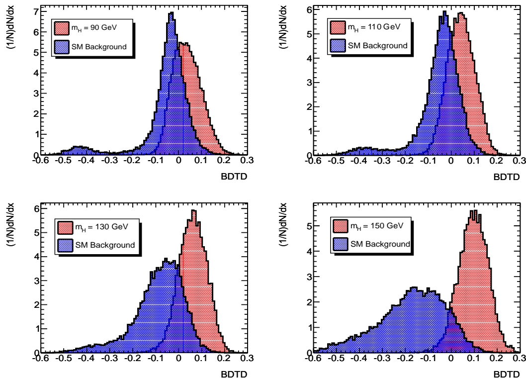
FIG. 8: BDTD response functions for pp \rightarrow t\bar{t}X , followed by the decay t \rightarrow W^+b (SM) and the decay chain t \rightarrow H^+b , with the SM background (in shaded blue) and the charged Higgs signal process (in shaded red) for four different charged Higgs masses.
