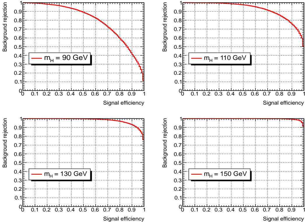
FIG. 18: SM background rejection vs. charged Higgs signal efficiency for the four charged Higgs masses indicated on the figure from the process pp \rightarrow t/\bar{t}X .
