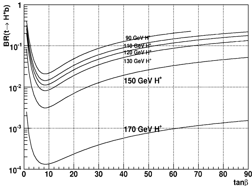
FIG. 1: Branching ratio \mathcal{B}(t \rightarrow H^+ b) in MSSM as a function of \tan\beta for the charged Higgs masses as indicated. (Figure taken from [44]).
