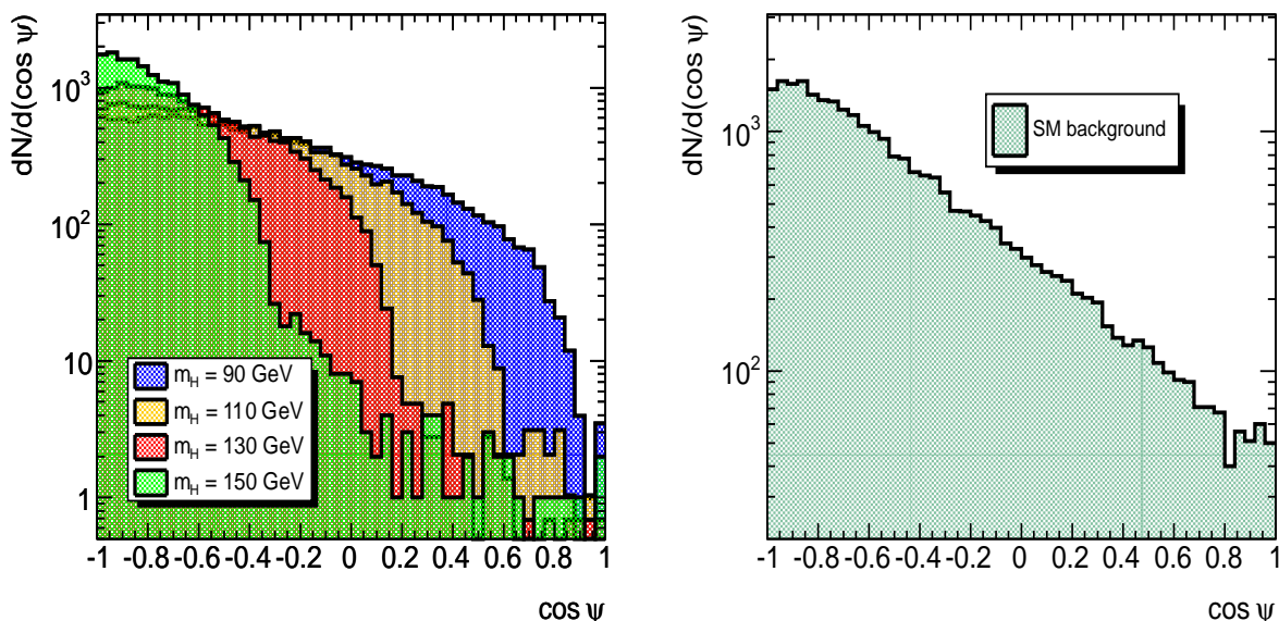
FIG. 3: The distribution dN/d \cos \psi for the t\bar{t} production as measured in the decay chain t \rightarrow bW \rightarrow b(\tau\nu_\tau) \rightarrow b(\rho\bar{\nu}_\tau)\nu_\tau (right-hand frame), and in t \rightarrow bH \rightarrow b(\tau\nu_\tau) \rightarrow b(\rho\bar{\nu}_\tau)\nu_\tau for four different charged Higgs masses, as indicated on the figure (left-hand frame).
