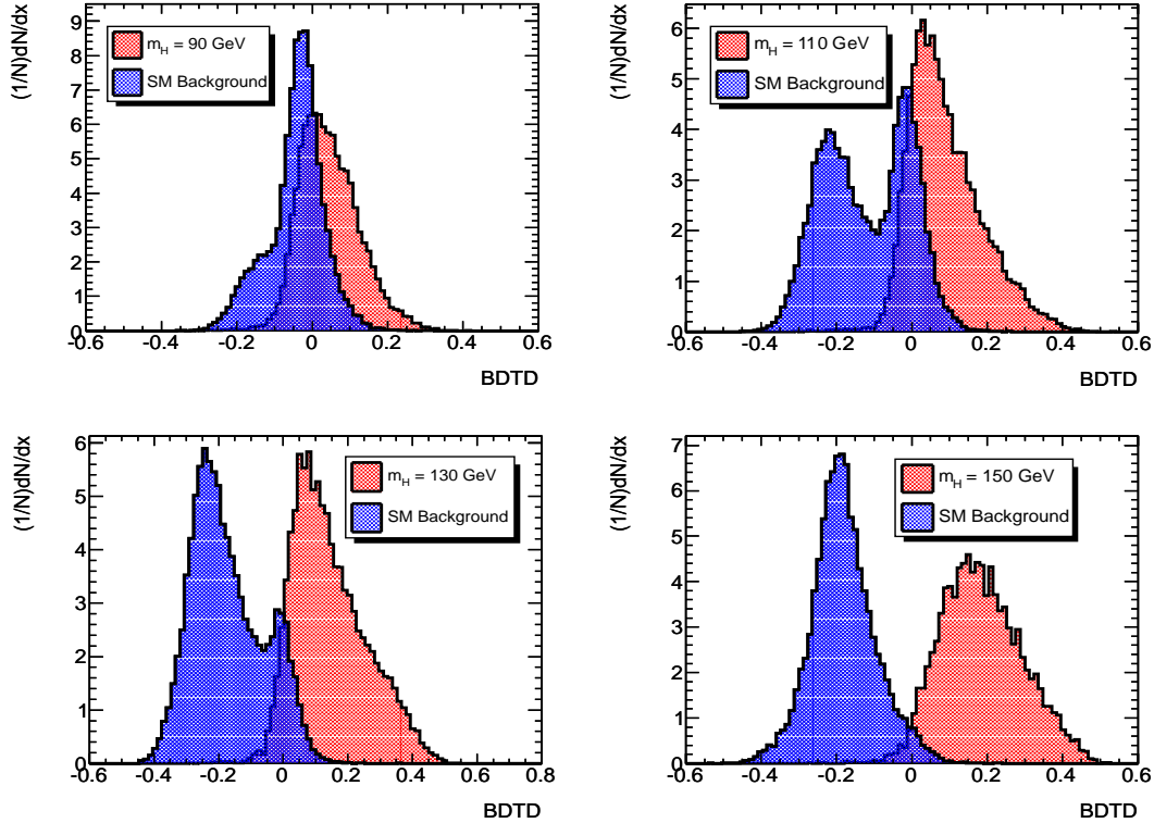
FIG. 17: BDTD response functions for pp \rightarrow t/\bar{t}X , followed by the decay t \rightarrow W^+b (SM) and the decay chain t \rightarrow H^+b , with the SM background (in shaded blue) and the charged Higgs signal process (in shaded red) for four different charged Higgs masses.
