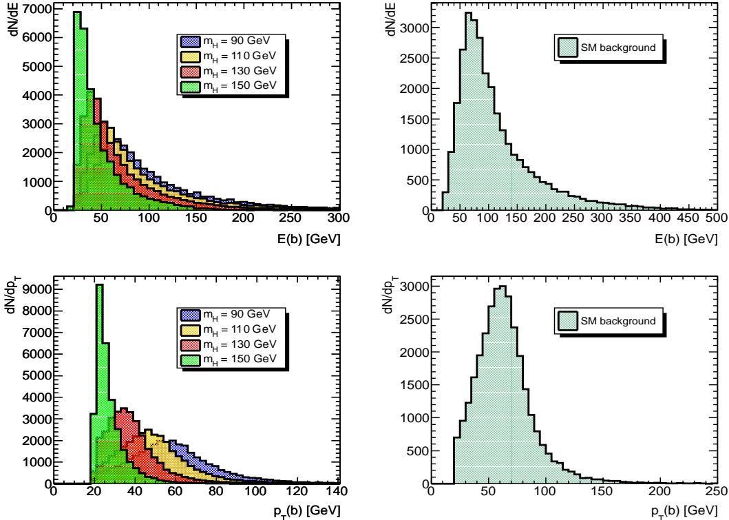
FIG. 12: Distributions in the energy of the b -jet, E(b) , and transverse momentum of the b -jet, p_T(b) from the process pp \rightarrow t/\bar{t}X , followed by the decay t \rightarrow W^+b (right-hand frames), and the same distributions for the decay chain t \rightarrow H^+b with the four indicated charged Higgs masses (left-hand frame).
