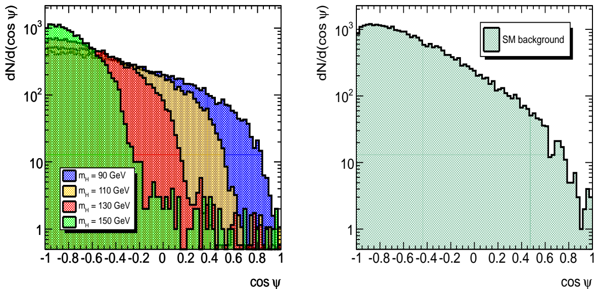
FIG. 11: The distribution dN/d\cos\psi for the pp \rightarrow t/\bar{t} + X production as measured in the decay chain t \rightarrow bW \rightarrow b(\tau\nu_\tau) \rightarrow b(\rho\bar{\nu}_\tau)\nu_\tau (right-hand frame), and in t \rightarrow bH \rightarrow b(\tau\nu_\tau) \rightarrow b(\rho\bar{\nu}_\tau)\nu_\tau for four different charged Higgs masses, as indicated on the figure (left-hand frame).
