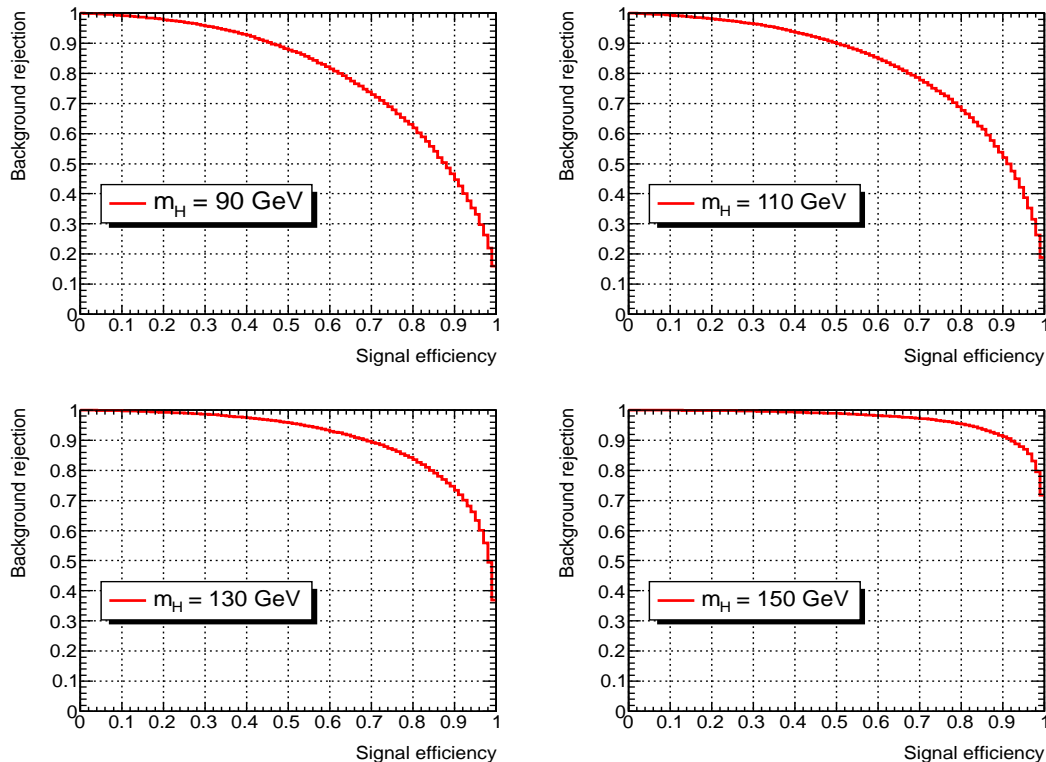
FIG. 9: SM background rejection vs. charged Higgs signal efficiency for the four charged Higgs masses indicated on the figure from the process pp \rightarrow t\bar{t}X .
