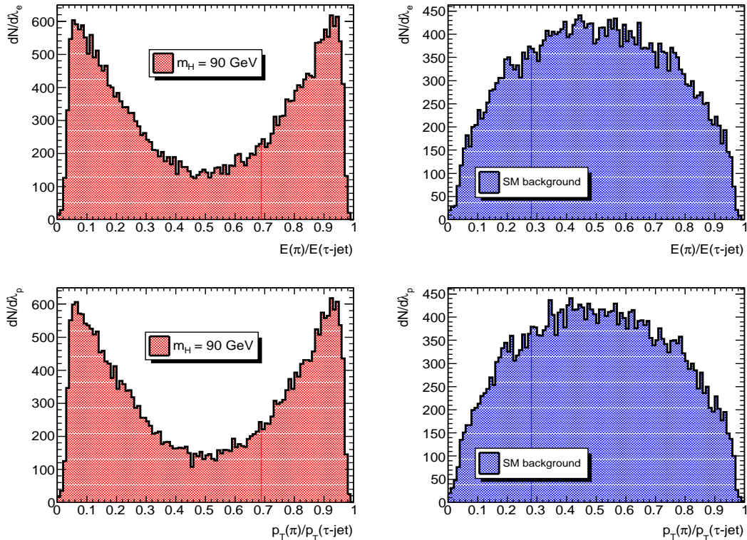
FIG. 15: Distributions in the fractional energy of the single-charged prong ( \pi^+ in \tau^+ -jet), E(\pi)/E(\tau - \text{jet}) , and in the transverse momentum of the single-charged prong, p_T(\pi)/p_T(\tau - \text{jet}) from the pp \rightarrow t/\bar{t}X , followed by the SM decay t \rightarrow W^+b (right-hand frames), and the same distributions for the decay chain t \rightarrow H^+b with the four indicated charged Higgs masses (left-hand frame).
