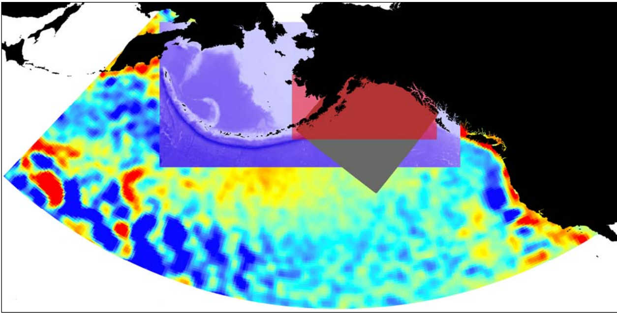
Figure 1: Extents of data sets described in this report. The largest extents include the entire eastern North Pacific and Bering Sea; the 9 \times 9 \text{ km}^2 study area (purple) includes the Gulf of Alaska and Bering Sea, while the 3 \times 3 \text{ km}^2 study area (red) includes the northern Gulf of Alaska. The extents of the Hermann circulation model are overlaid in grey.
