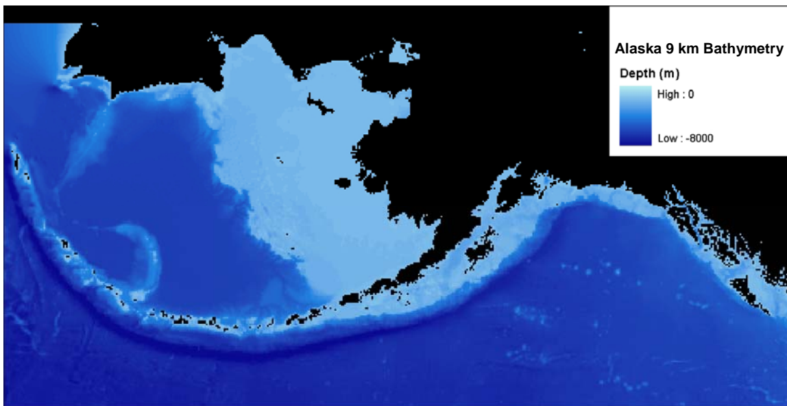
Figure 2: Bathymetry for the 9x9 km 2 Bering Sea / Gulf of Alaska study area.
