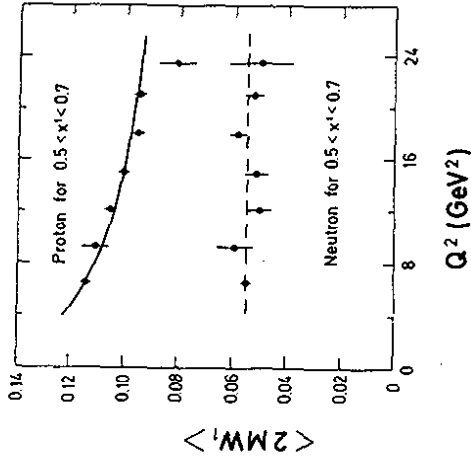
Fig. 5.14. Comparison of the experimental data 84 with the predicted variation of F_{NS} = F_1^{ep} - F_1^{en} in Eq. (5.63), using the neutron data as input. 83
