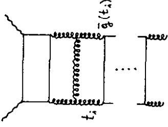
Fig. 6.8. Bethe-Salpeter ladder contributing to the Q^2 dependence of singlet structure functions.
