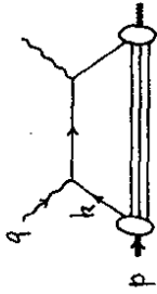
Fig. 5.2. Deep inelastic scattering in the (naive) parton model: The hand-bag diagram.
