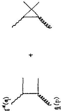
Fig. 6.2. Diagrams giving rise to F_2^g \sim P_{qg} and F_L^g .
