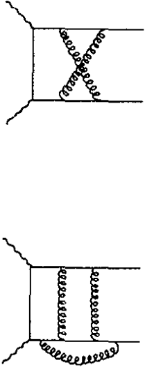
Fig. 6.5. A sample of diagrams which do not contribute to the leading log approximation.
