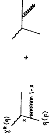
Fig. 6.3. Diagrams giving rise to F_2^q \sim P_{qq} , P_{gq} and F_L^q .
