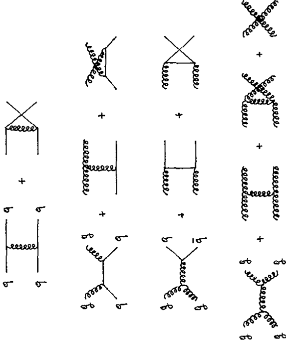
Fig. 11.1. Examples of lowest-order subprocesses d\sigma^{ab} \rightarrow cd contributing to the high- p_T process in Eq. (11.1).
