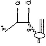
Fig. 5.17. Bethe-Heitler process for heavy-quark production.
