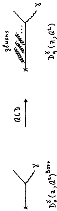
Fig. 5.26. QCD corrections to the q \rightarrow \gamma Born term.
