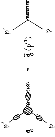
Fig. 6.7. Virtual corrections that make the coupling constant run.
