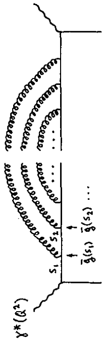
Fig. 10.3. Rainbow diagrams ( s_i > s_{i+1} ) giving rise to the Q^2 dependence of D_q^h(z, Q^2) .
