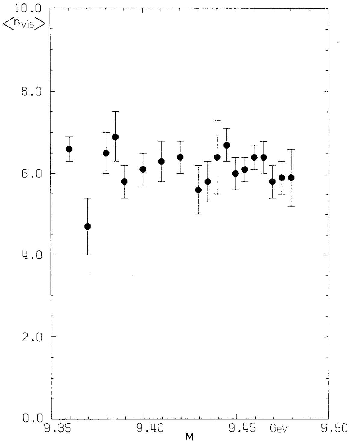
Fig. 2 Average multiplicities as found in the visual scan of the selected events (charged particles + photons).
