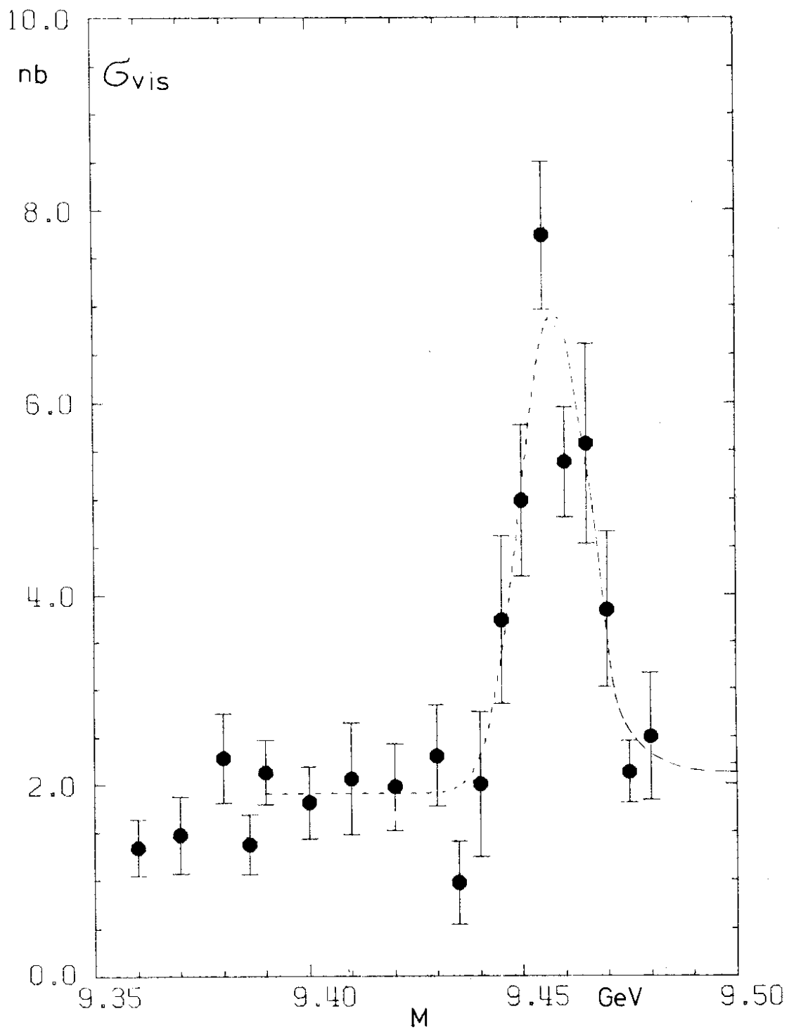
Fig. 1 Visible cross section of the reaction e^+e^- \rightarrow hadrons as defined by the trigger and the selection criteria. The dashed curve represents the best fit including gaussian resolution and radiative corrections.
