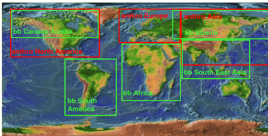
Figure 9: Region boundaries for the tagged CO tracer simulations with the ECHAM-5 model. Fossil fuel combustion emission regions are marked red, those from biomass burning are marked in green.
