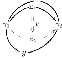
Figure 9: A 3-morphism in a 3-path 3-category: a volume V , cobounding two surfaces \Sigma_1 and \Sigma_2 , which each cobound two paths \gamma_1 and \gamma_2 which each cobound two points x any y .
