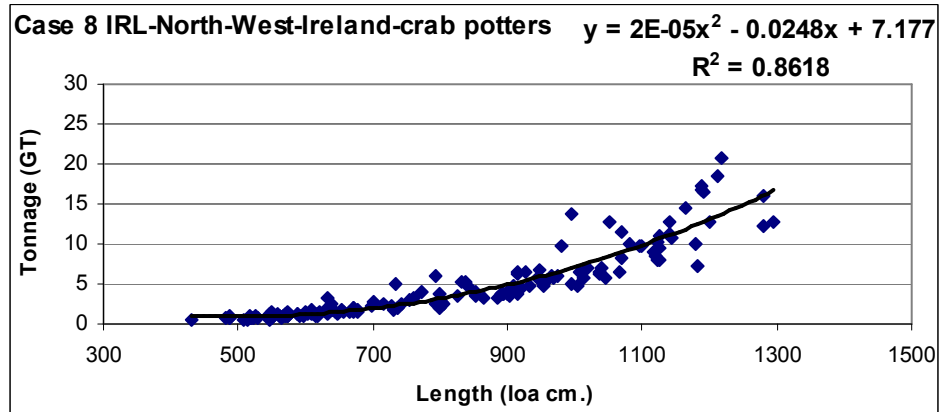
Figure 4.8-8 - Correlation between tonnage (GT) and length (loa cm.)
